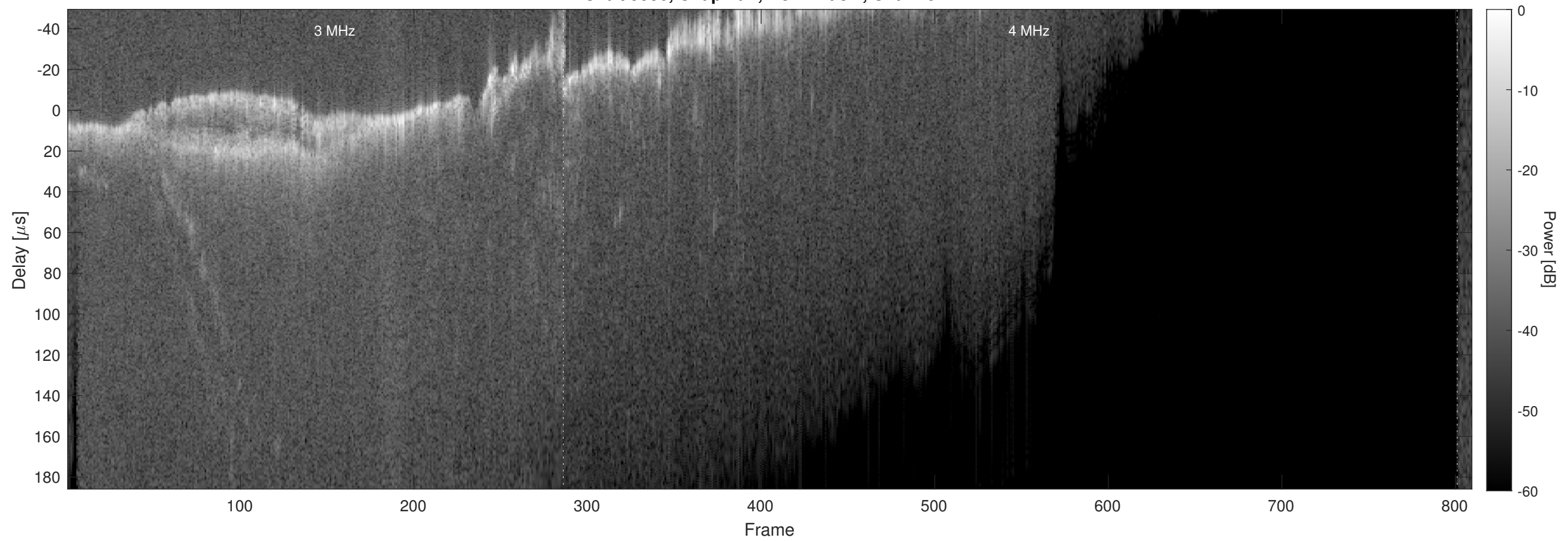
Orbit 9536, Chapman, No Window, Channel 2
