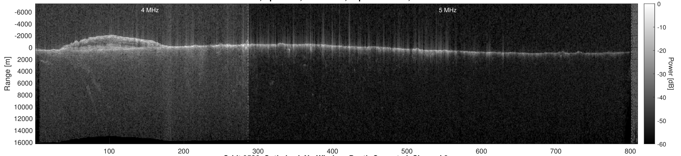
Orbit 9536, Optimized, No Window, Depth-Corrected, Channel 2
