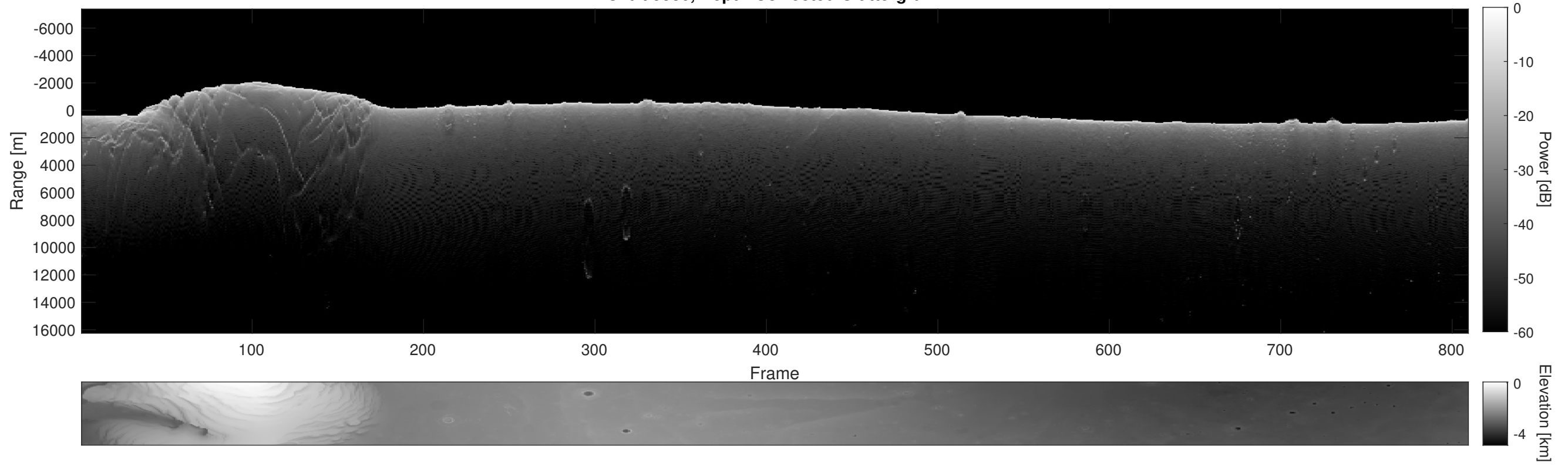
Orbit 9536, Depth-Corrected Cluttergram
