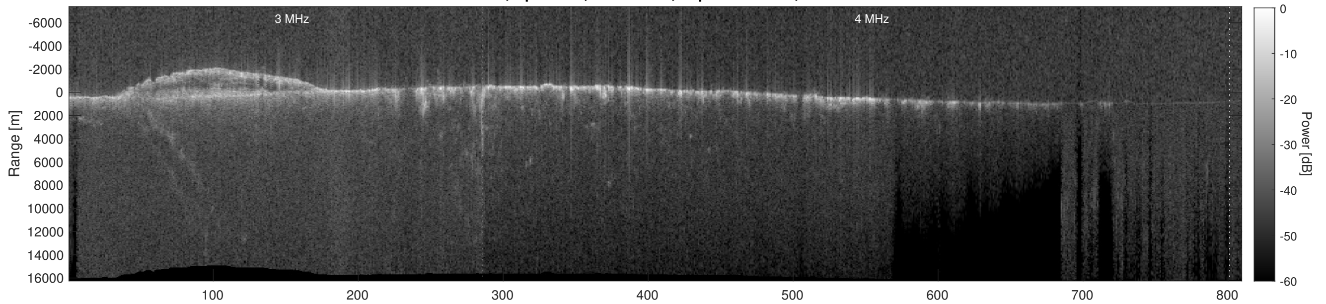
Orbit 9536, Depth-Corrected Cluttergram
