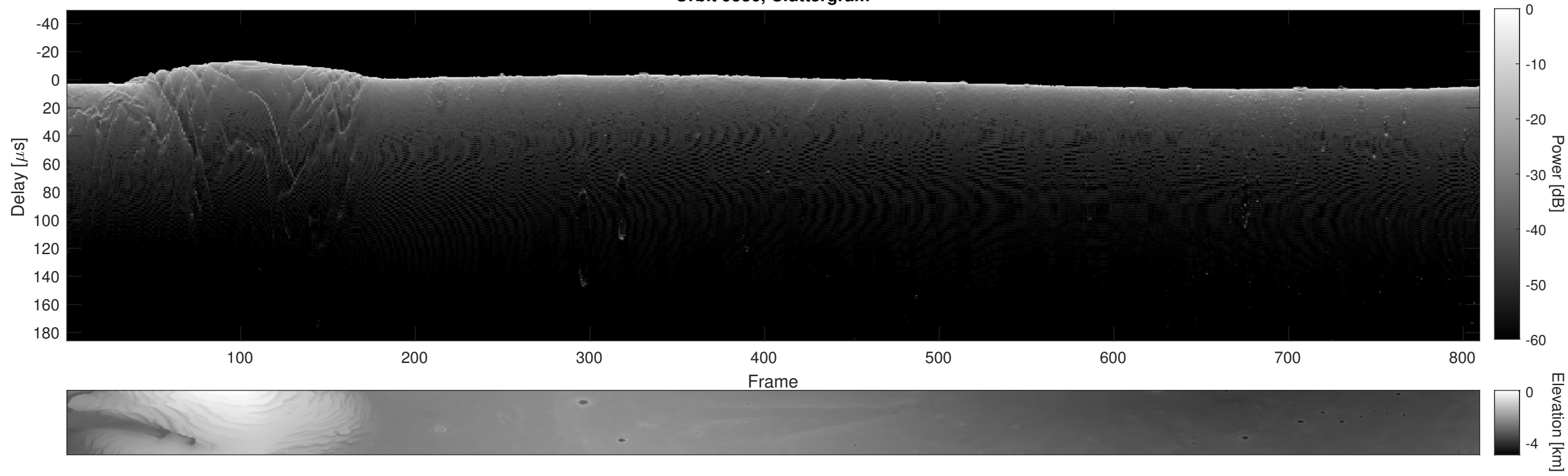
Orbit 9536, Cluttergram
