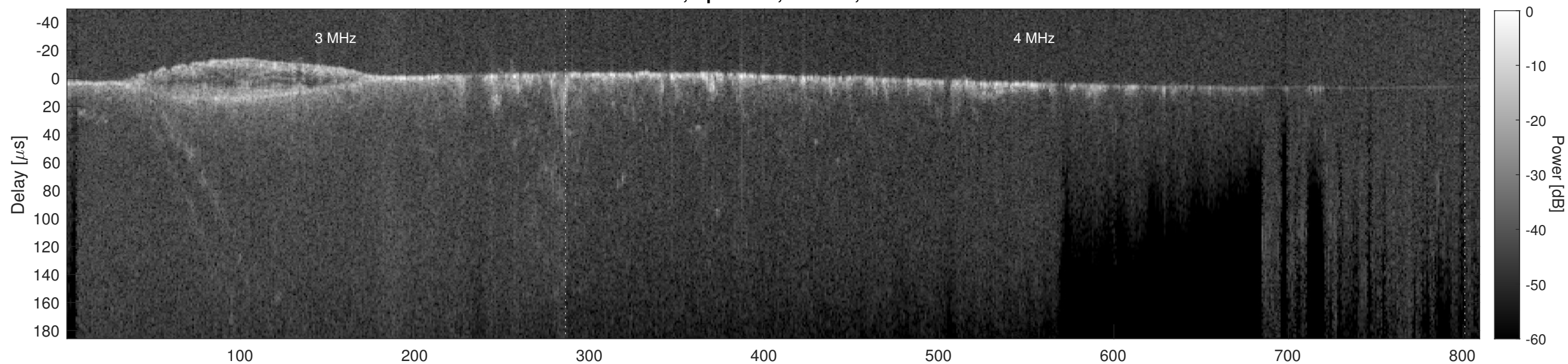
Orbit 9536, Cluttergram
