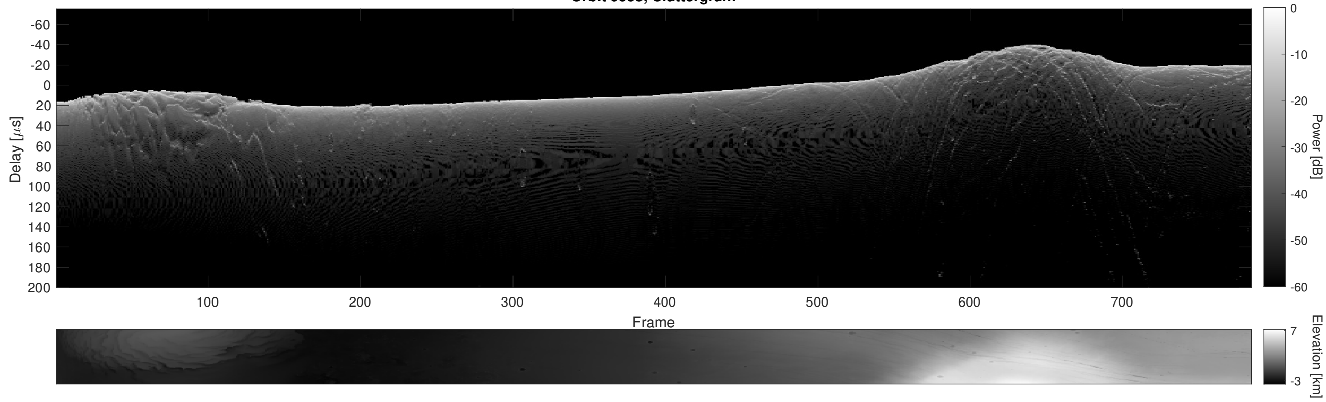
Orbit 9538, Cluttergram
