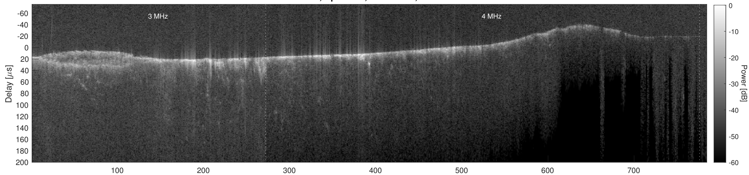
Orbit 9538, Cluttergram
