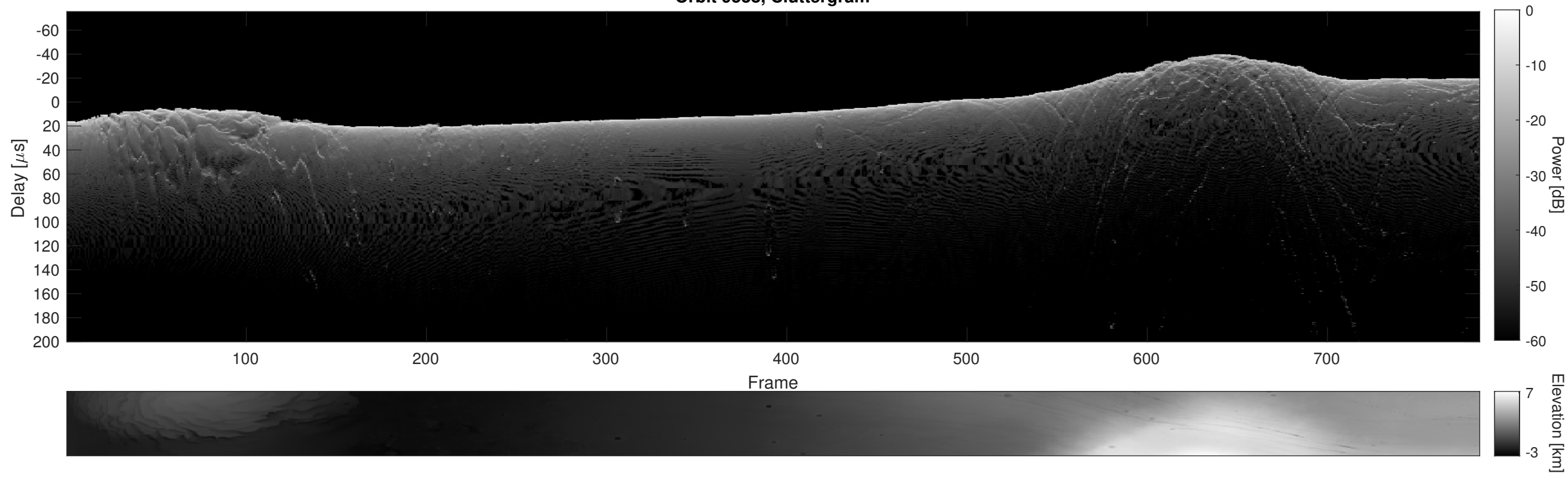
Orbit 9538, Cluttergram
