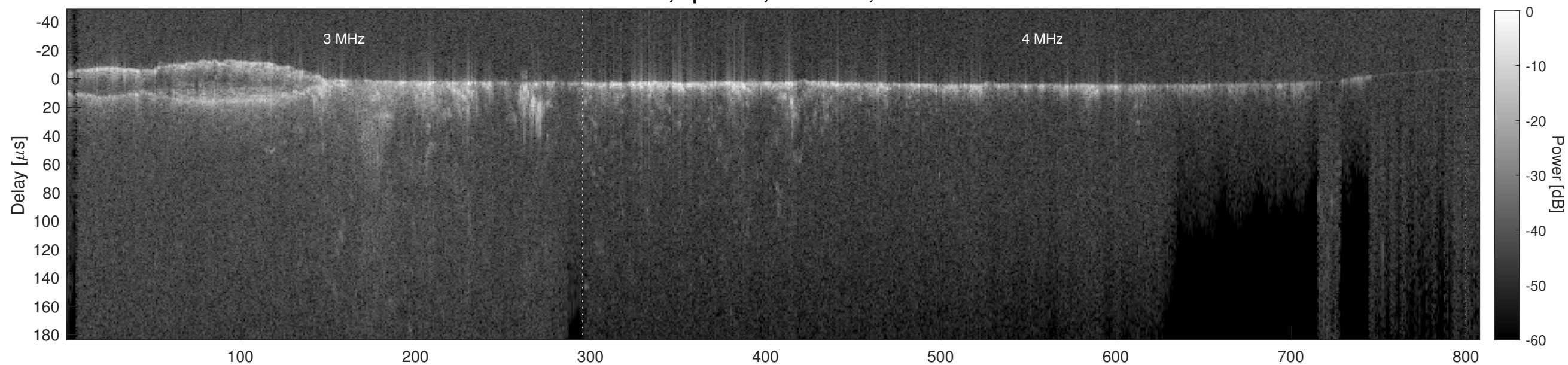
Orbit 9539, Cluttergram
