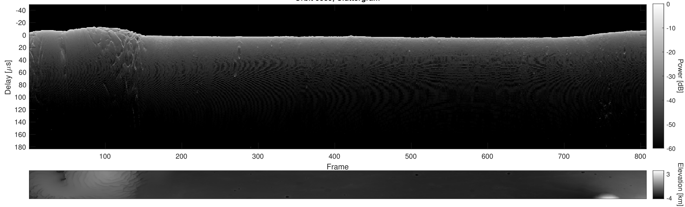
Orbit 9539, Cluttergram
