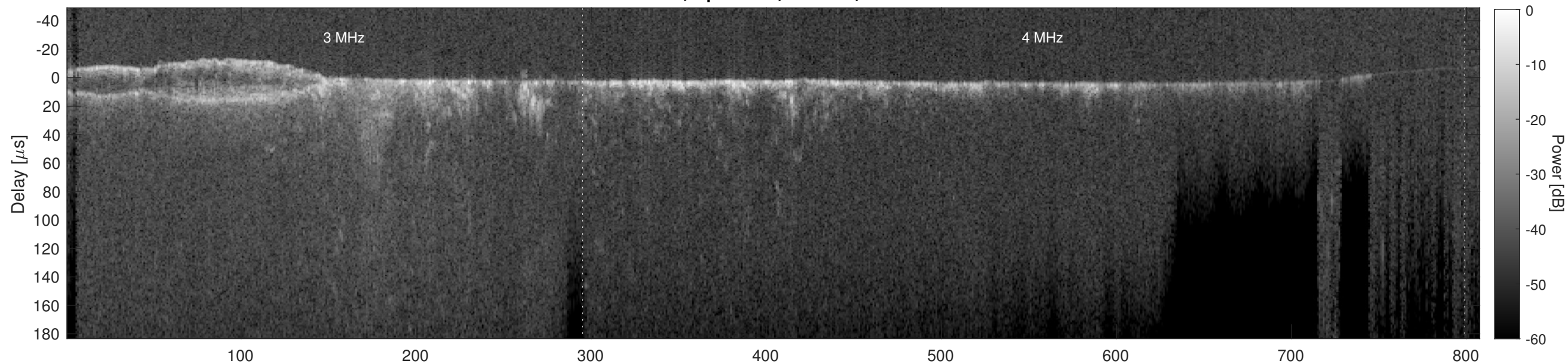
Orbit 9539, Cluttergram
