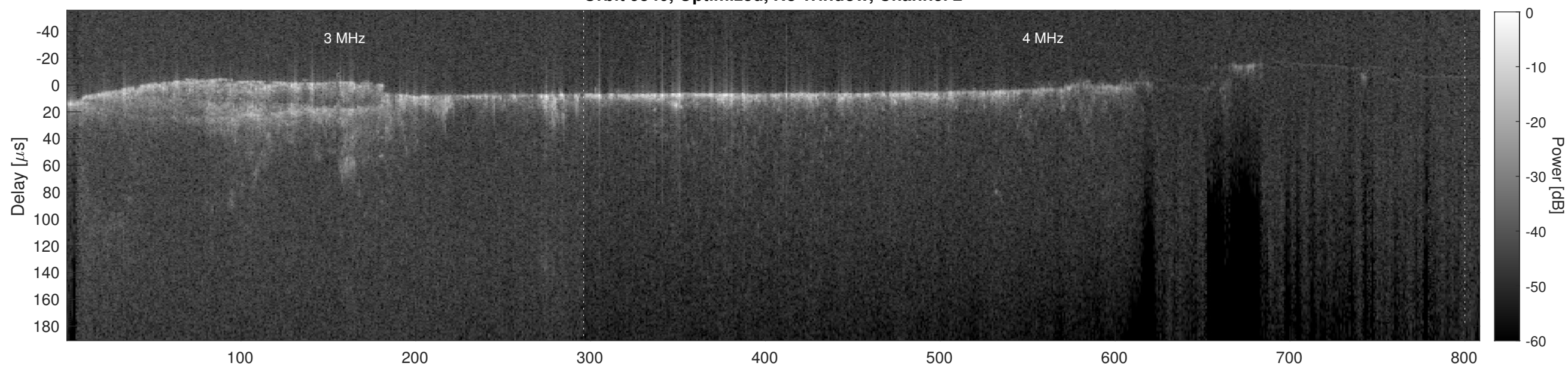
Orbit 9540, Cluttergram
