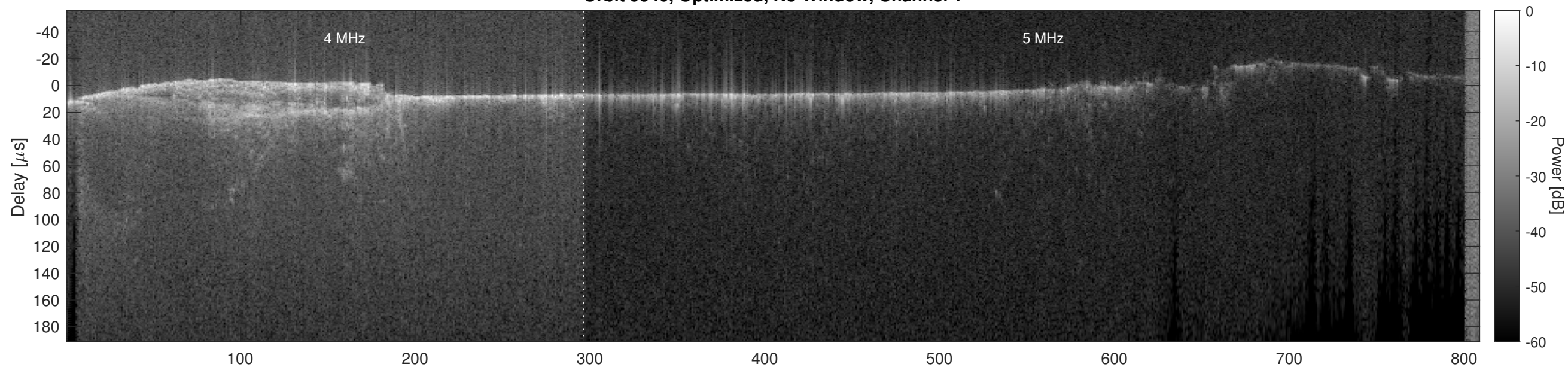
Orbit 9540, Optimized, No Window, Channel 2
