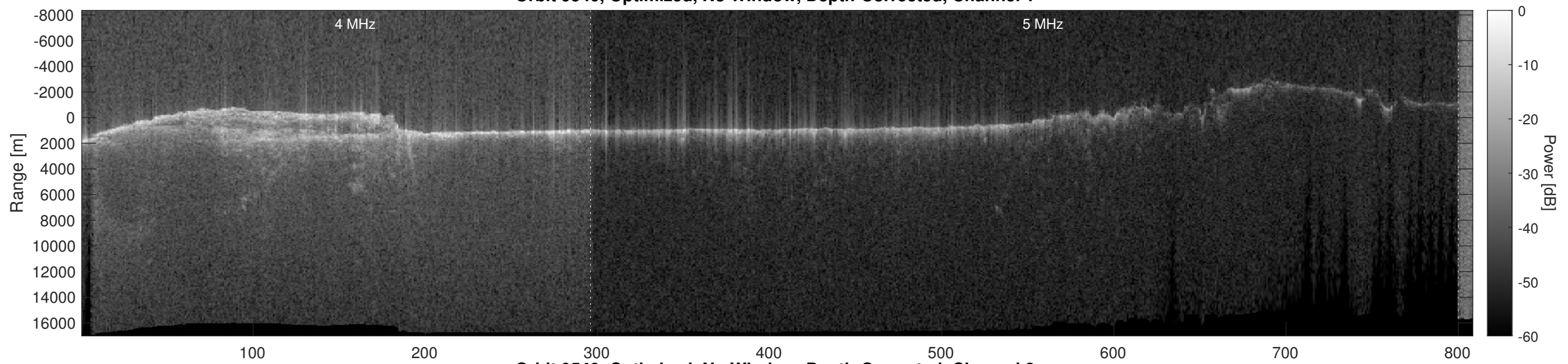
Orbit 9540, Optimized, No Window, Depth-Corrected, Channel 2
