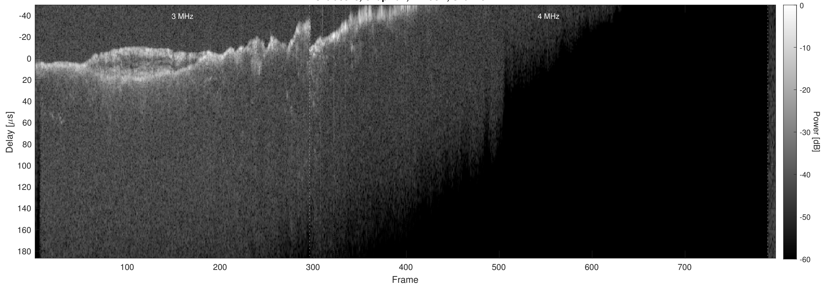
Orbit 9543, Chapman, Window, Channel 2
