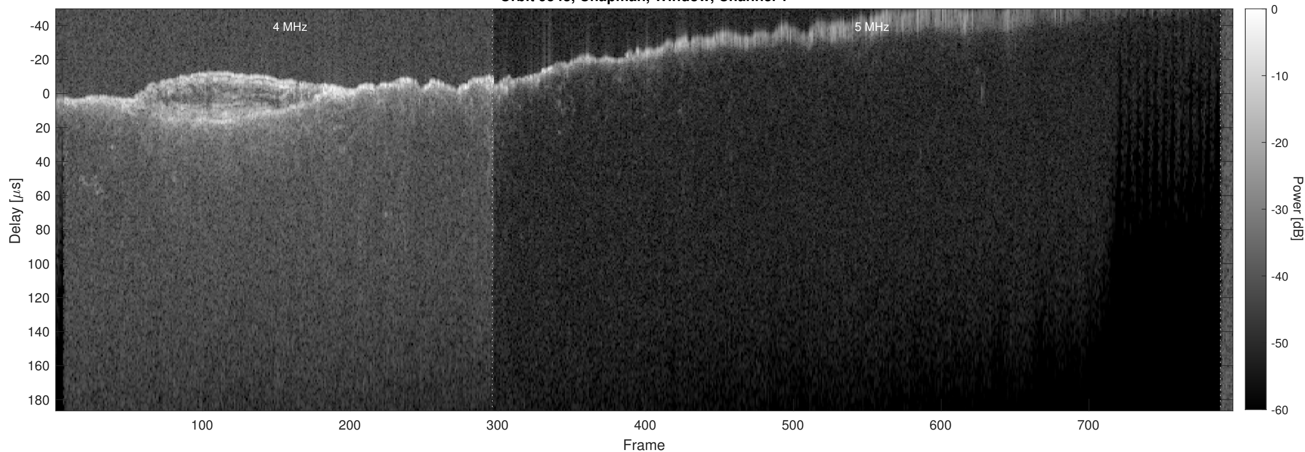
Orbit 9543, Chapman, Window, Channel 2
