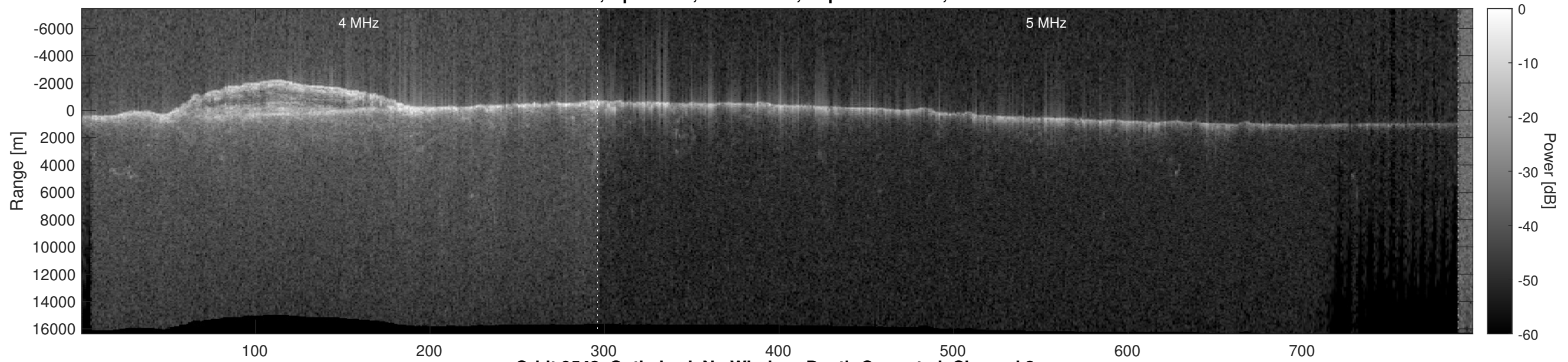
Orbit 9543, Optimized, No Window, Depth-Corrected, Channel 2
