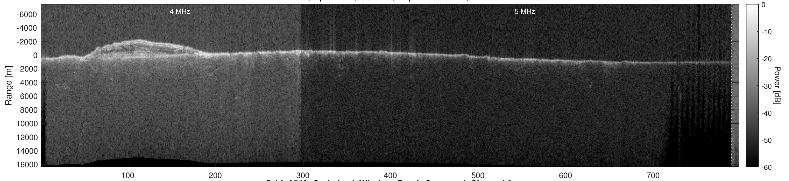
Orbit 9543, Optimized, Window, Depth-Corrected, Channel 2
