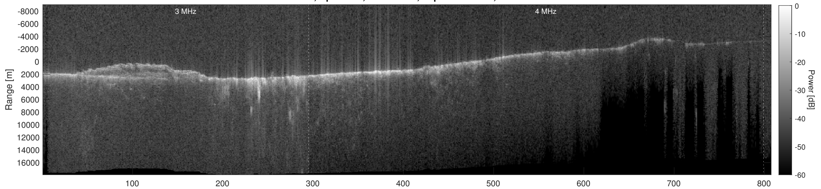
Orbit 9545, Depth-Corrected Cluttergram
