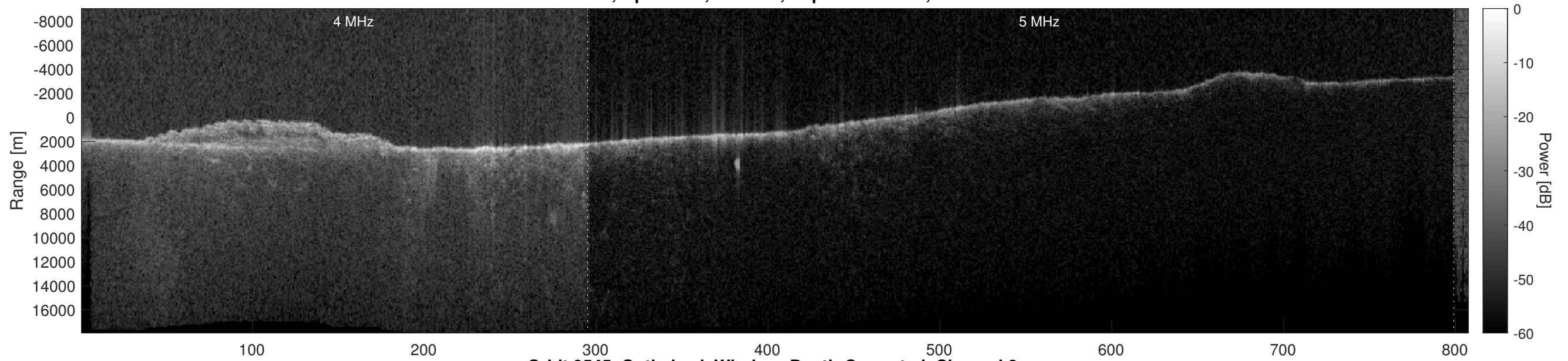
Orbit 9545, Optimized, Window, Depth-Corrected, Channel 2
