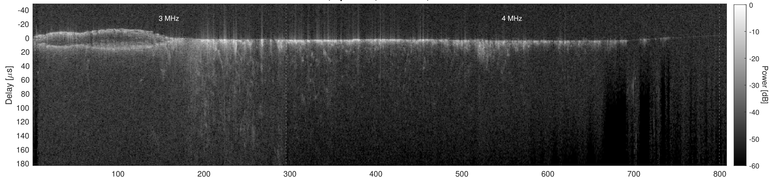
Orbit 9546, Cluttergram
