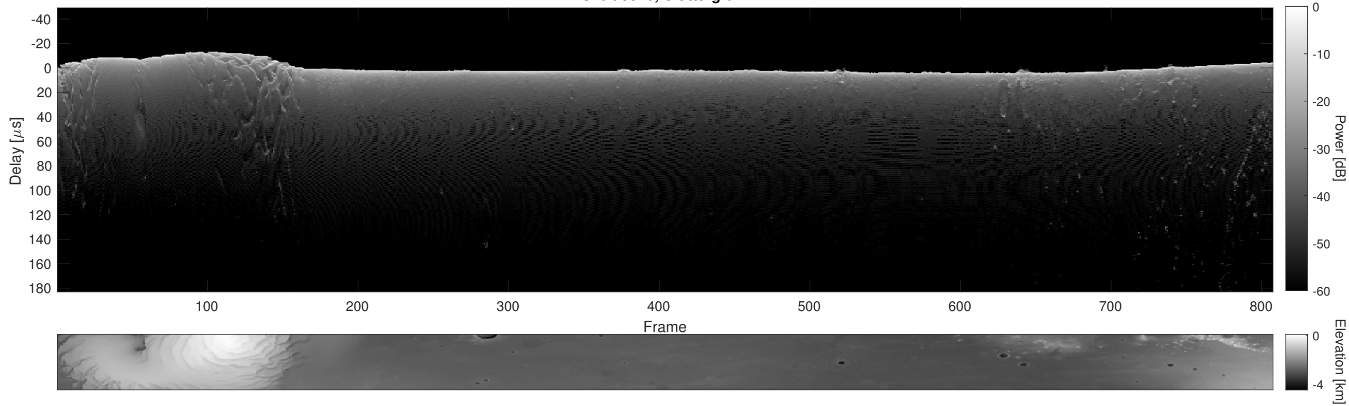
Orbit 9546, Cluttergram
