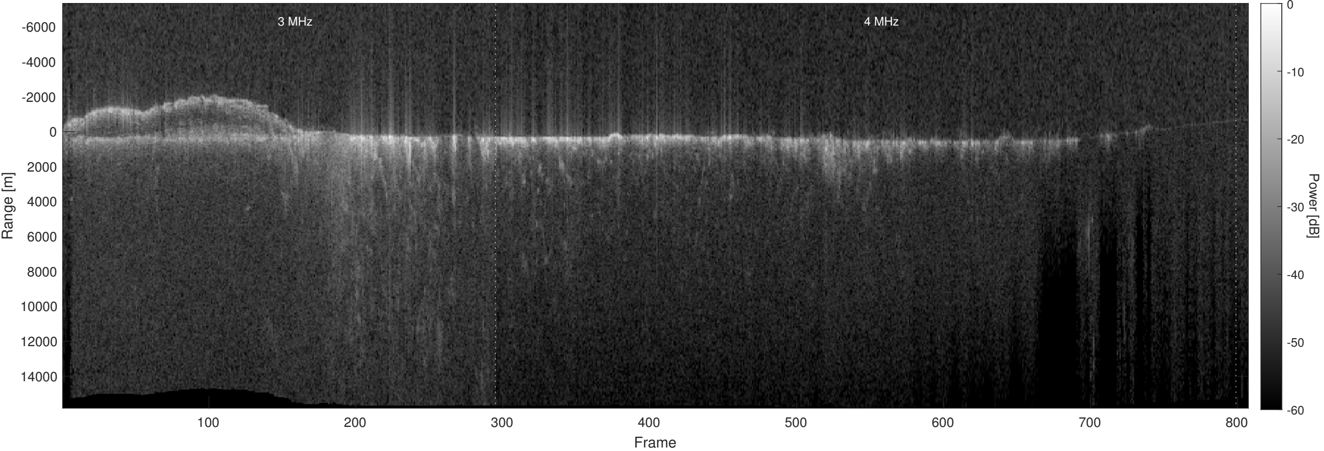
Orbit 9546, Optimized, No Window, Depth-Corrected, Channel 2
