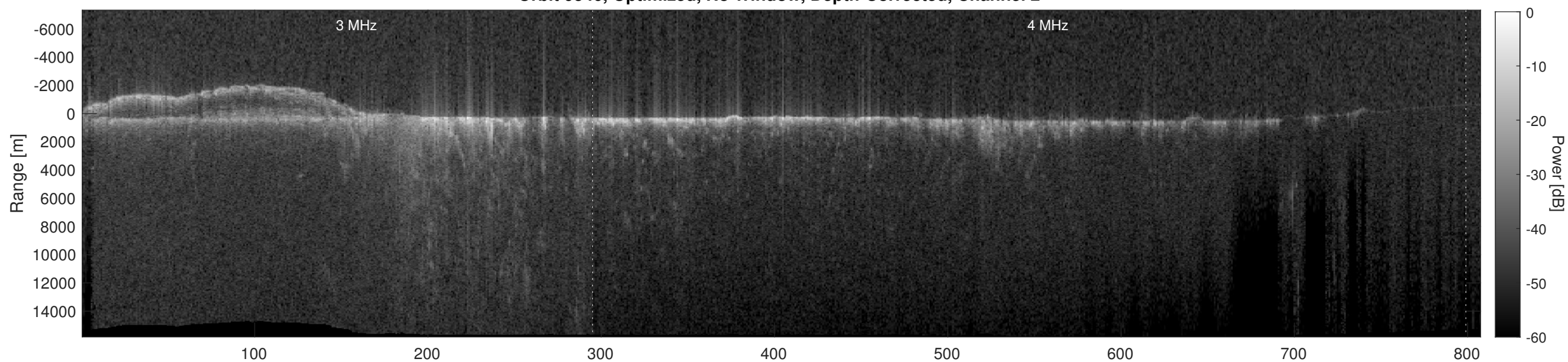
Orbit 9546, Depth-Corrected Cluttergram
