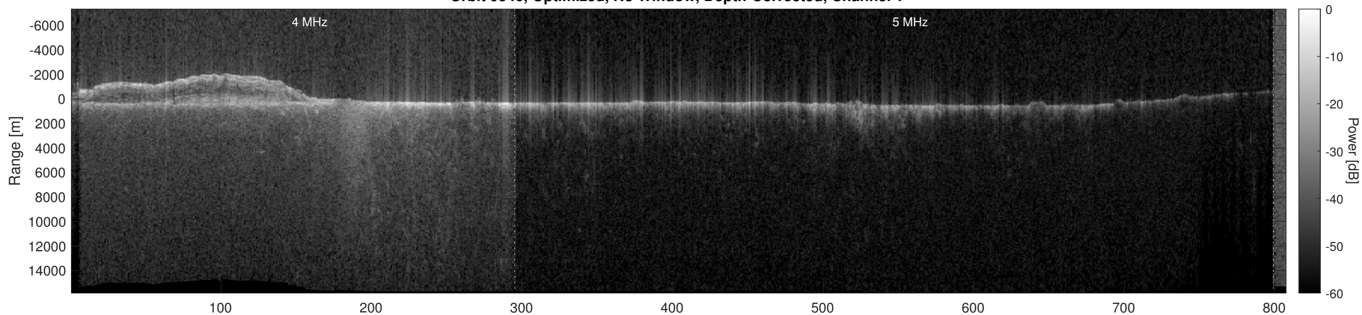
Orbit 9546, Optimized, No Window, Depth-Corrected, Channel 2
