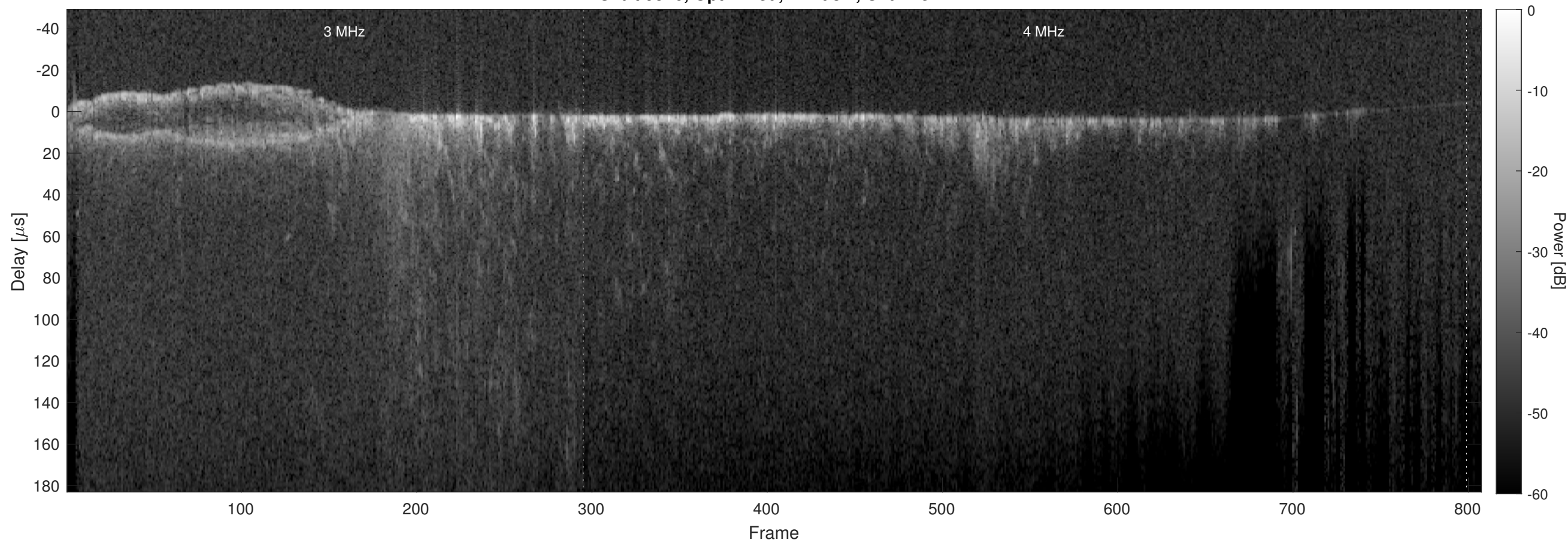
Orbit 9546, Optimized, Window, Channel 2
