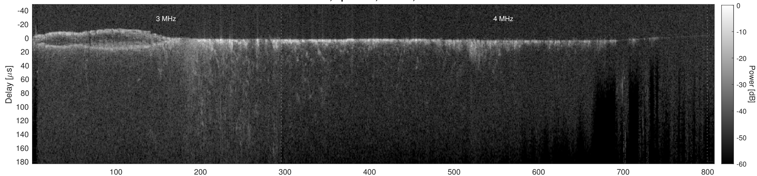
Orbit 9546, Cluttergram
