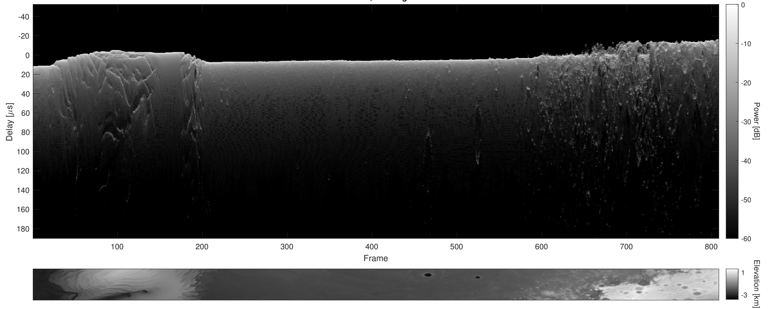
Orbit 9547, Cluttergram
