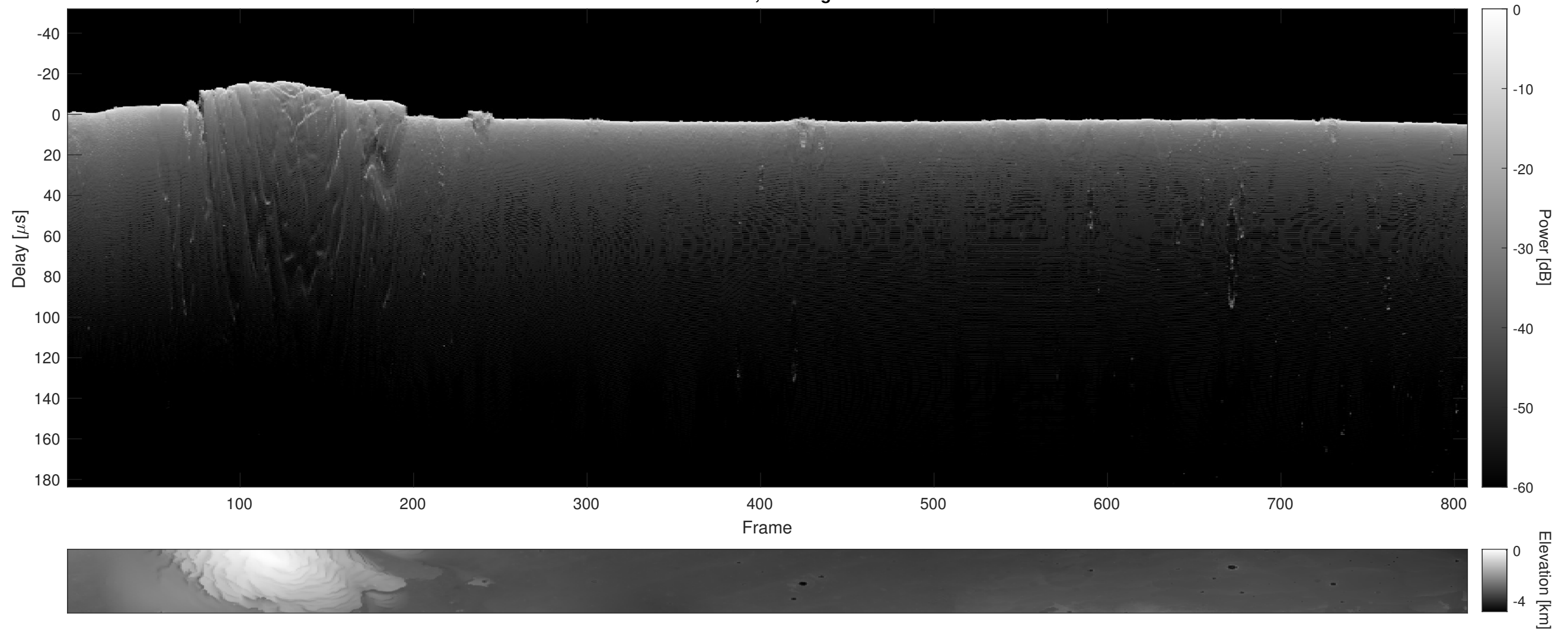
Orbit 9548, Cluttergram
