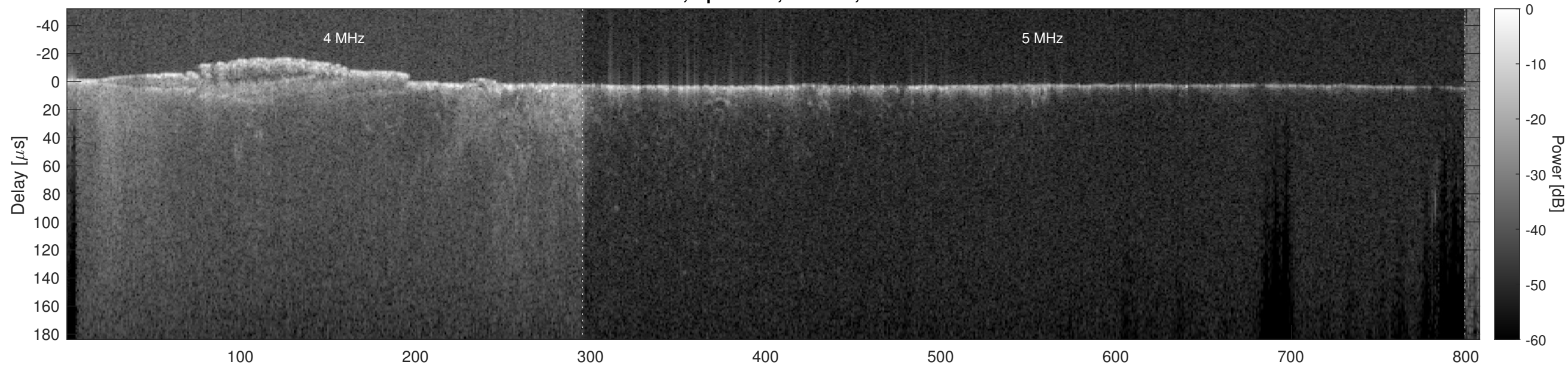
Orbit 9548, Optimized, Window, Channel 2
