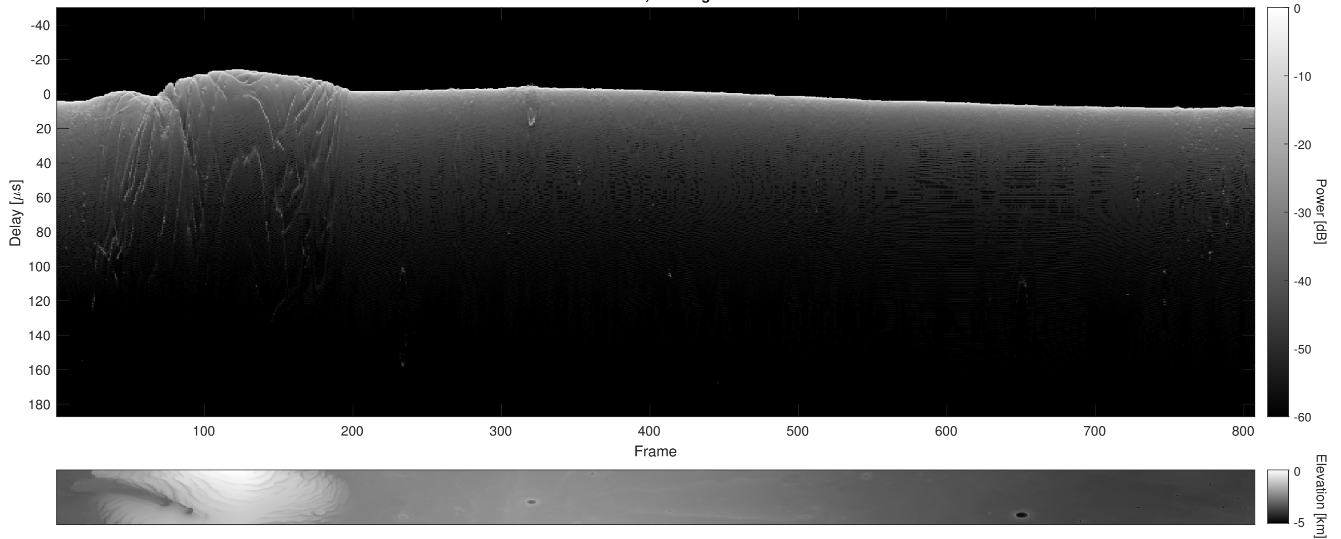
Orbit 9550, Cluttergram
