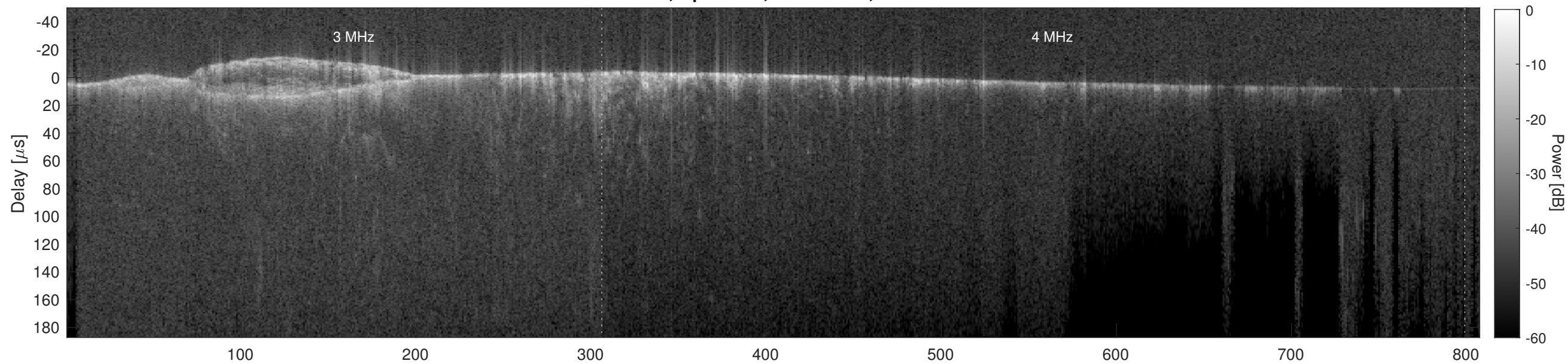
Orbit 9550, Cluttergram
