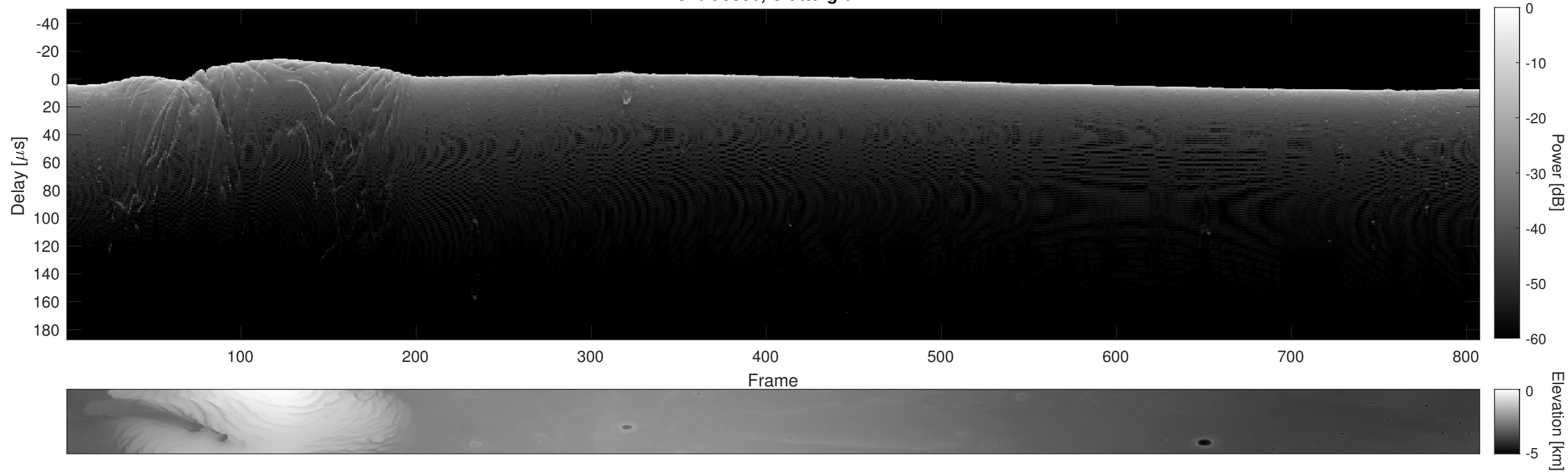
Orbit 9550, Cluttergram
