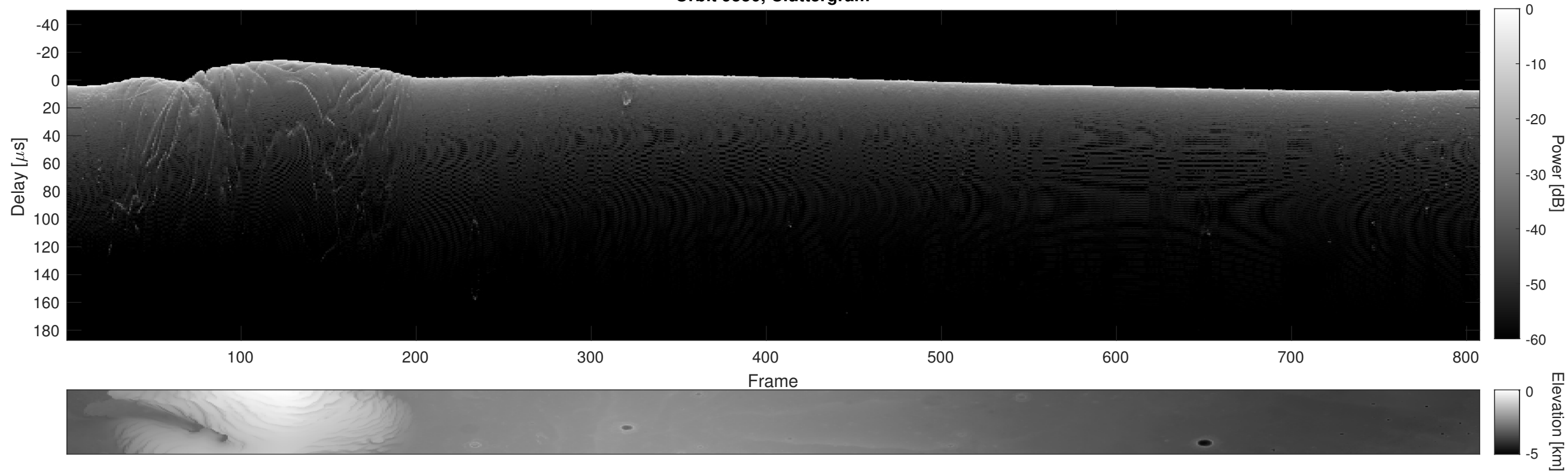
Orbit 9550, Cluttergram
