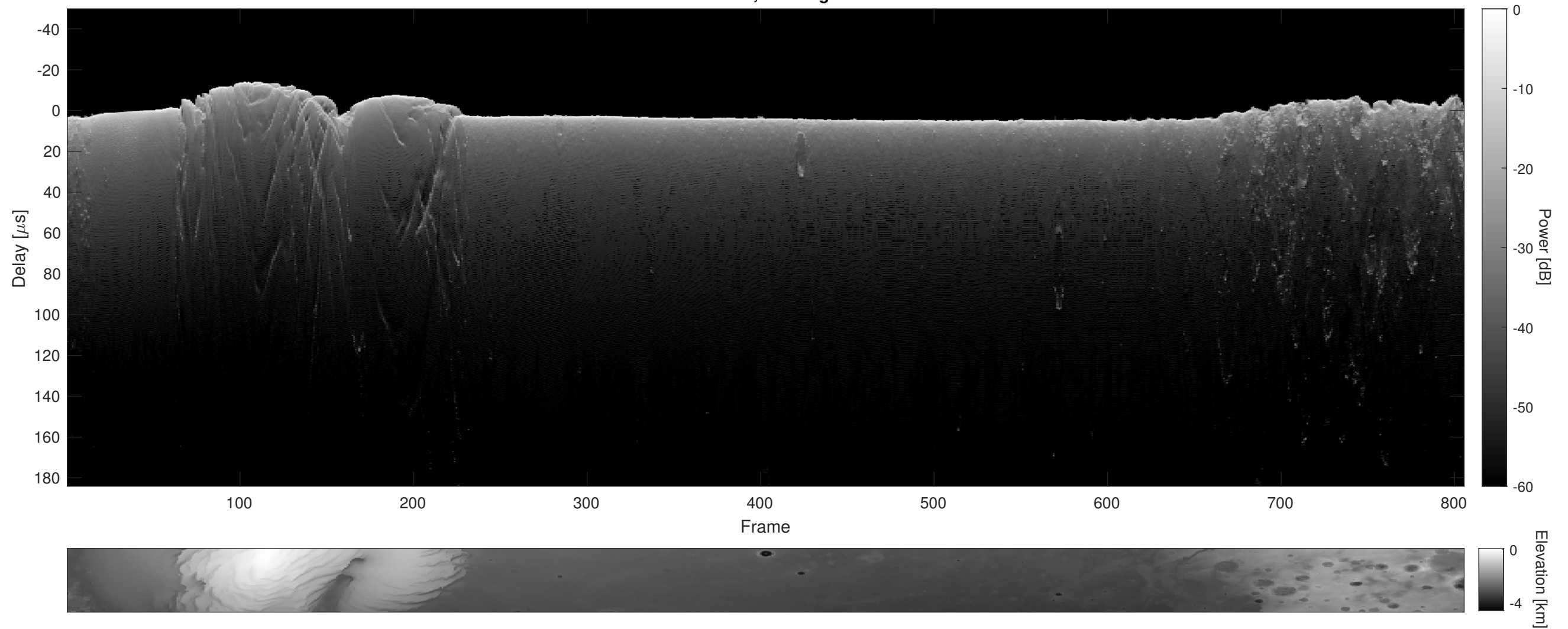
Orbit 9551, Cluttergram
