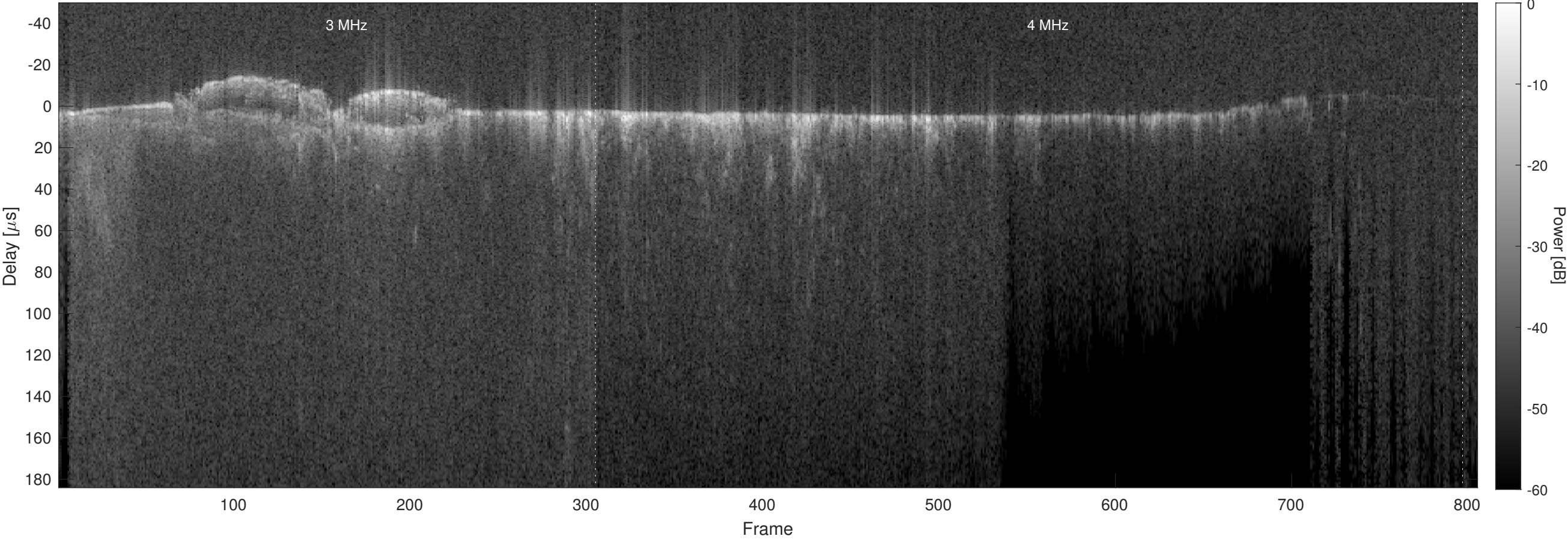
Orbit 9551, Optimized, No Window, Channel 2
