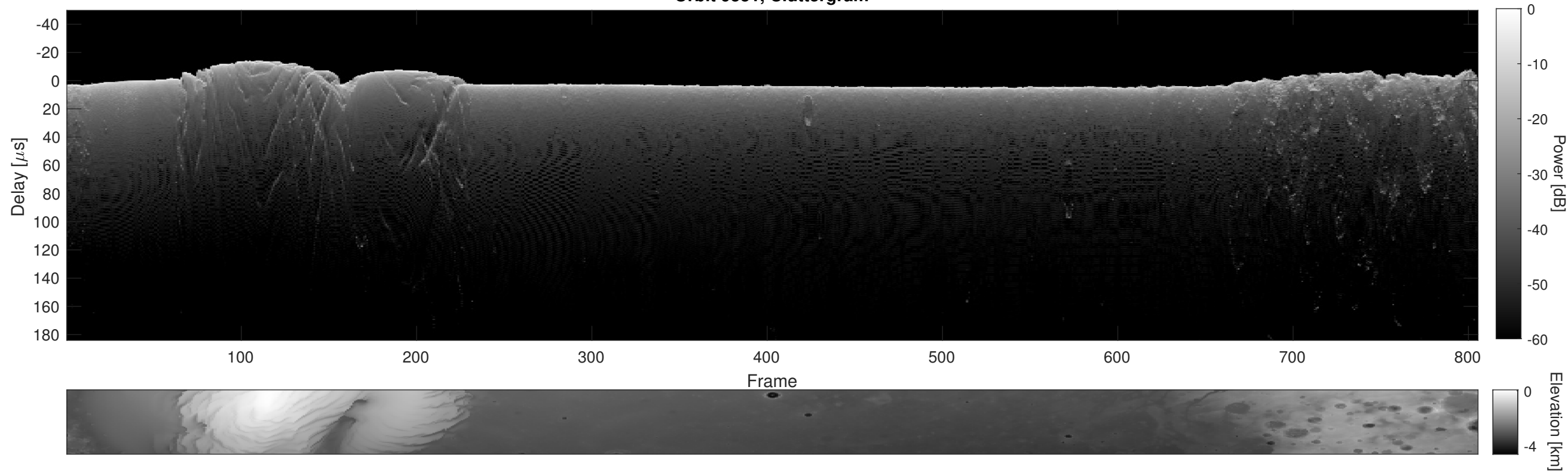
Orbit 9551, Cluttergram
