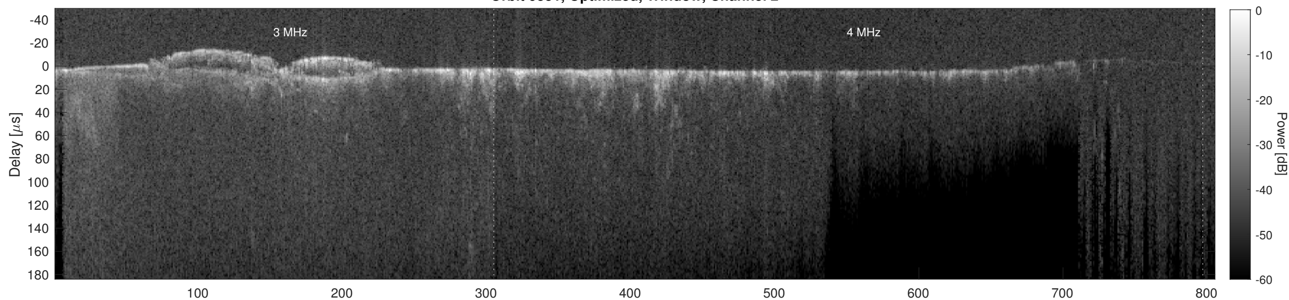
Orbit 9551, Cluttergram
