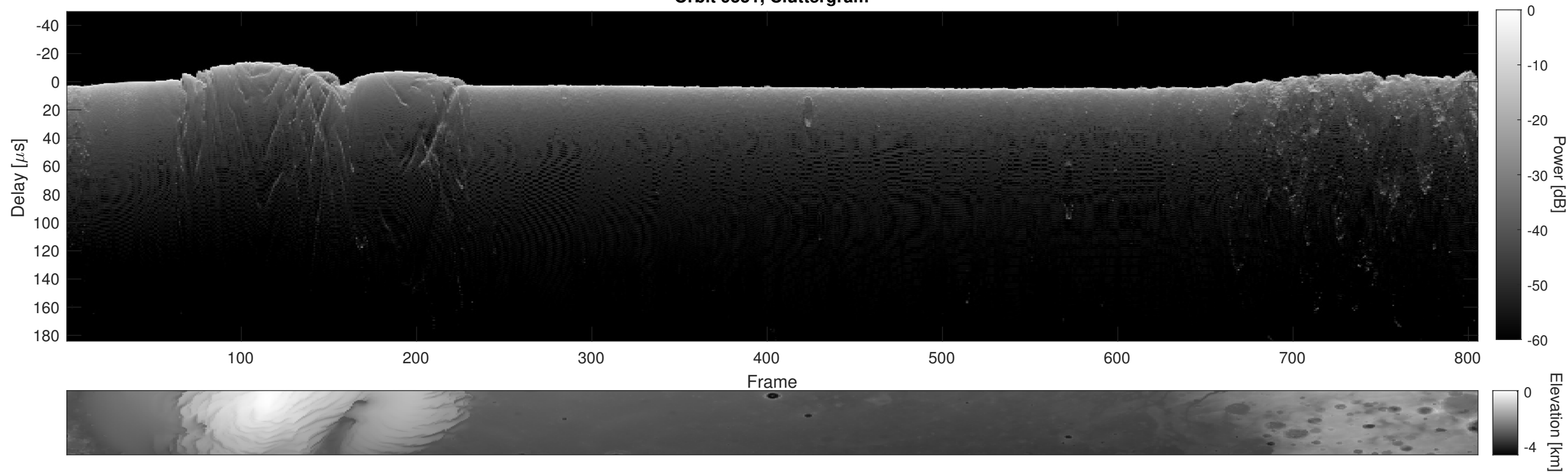
Orbit 9551, Cluttergram
