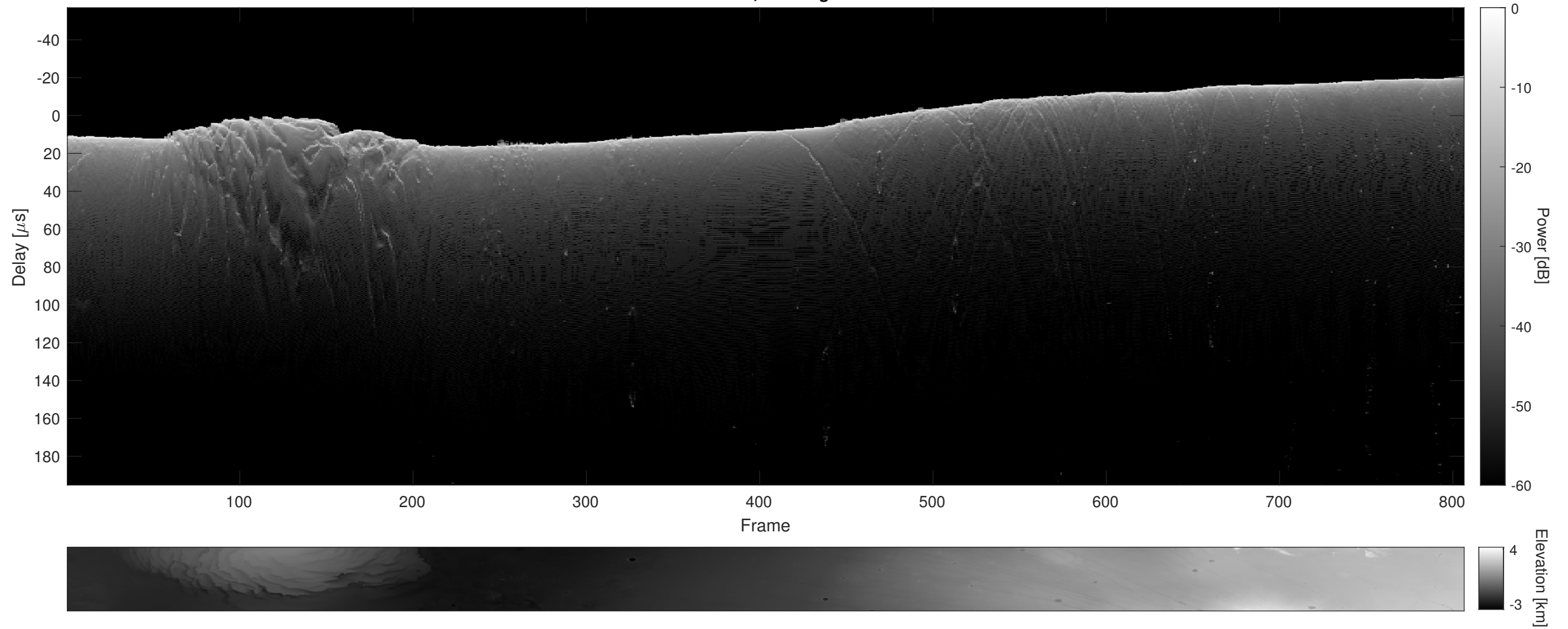
Orbit 9552, Cluttergram
