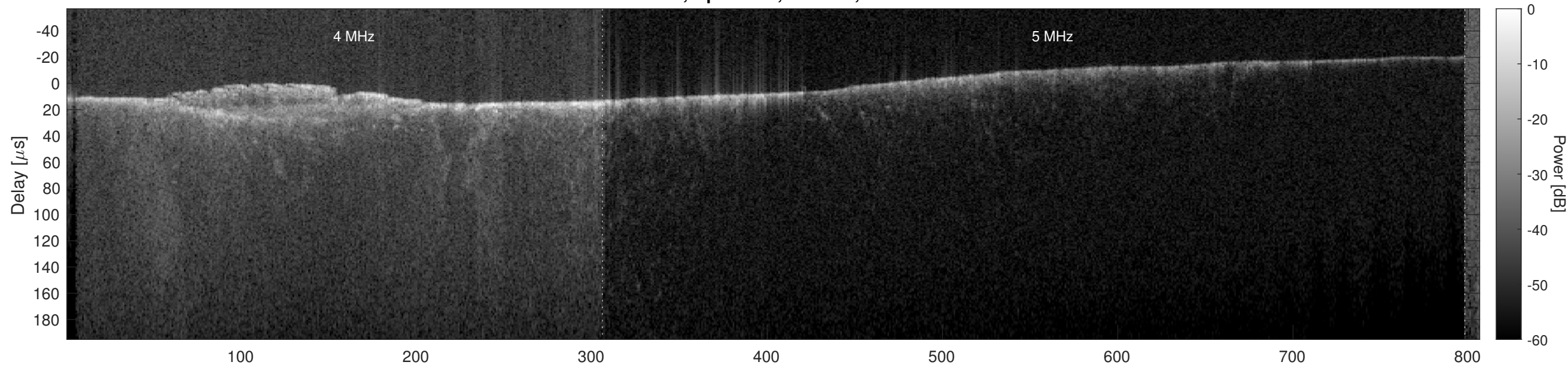
Orbit 9552, Optimized, Window, Channel 2
