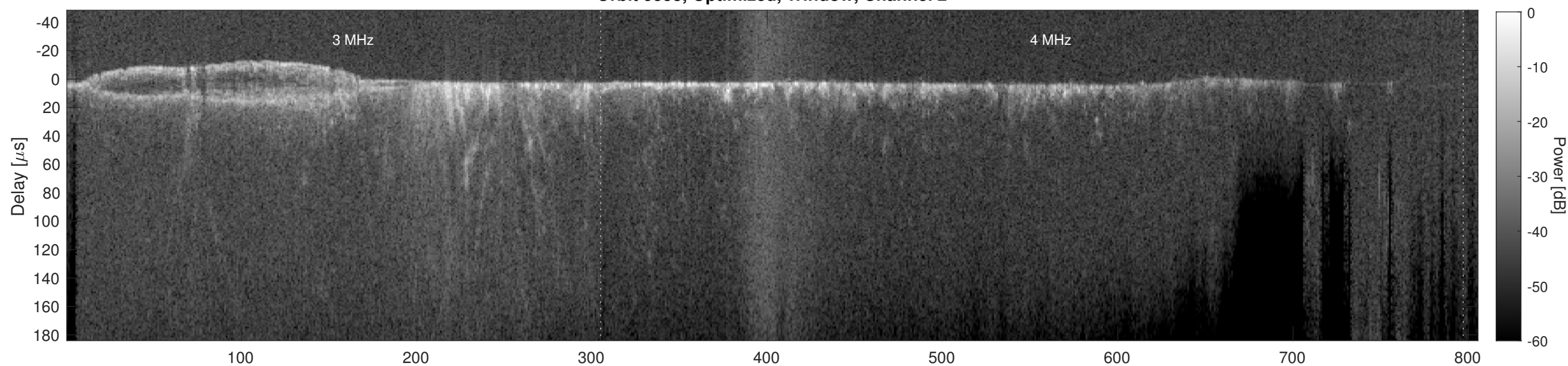
Orbit 9553, Cluttergram
