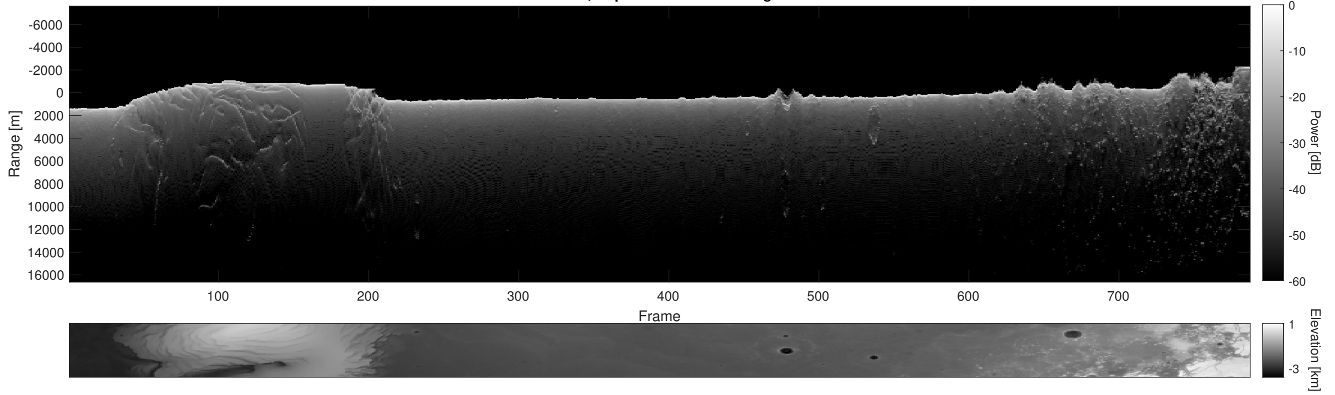
Orbit 9554, Depth-Corrected Cluttergram
