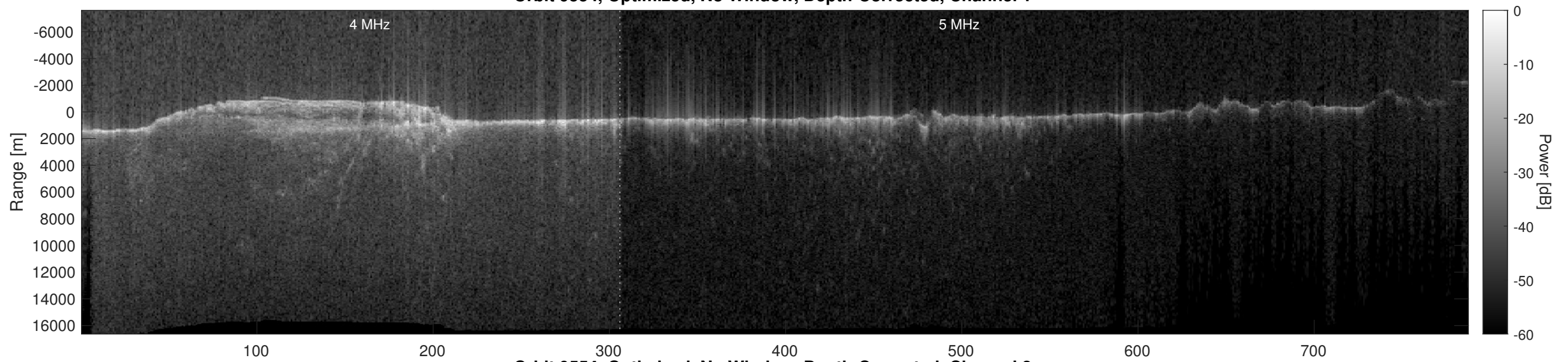
Orbit 9554, Optimized, No Window, Depth-Corrected, Channel 2
