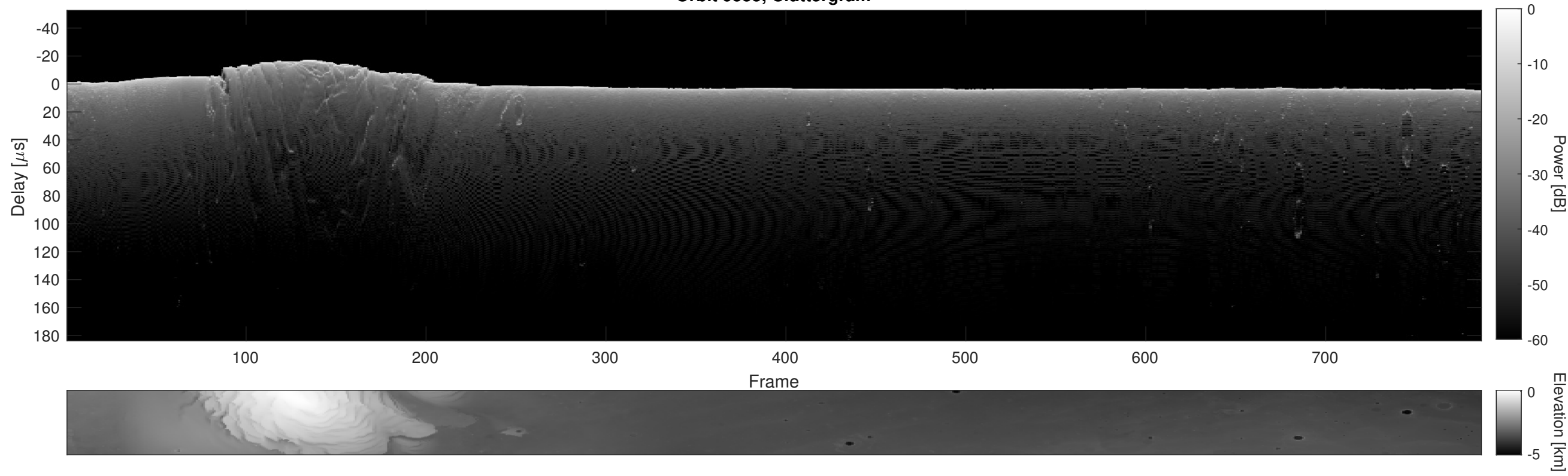
Orbit 9555, Cluttergram
