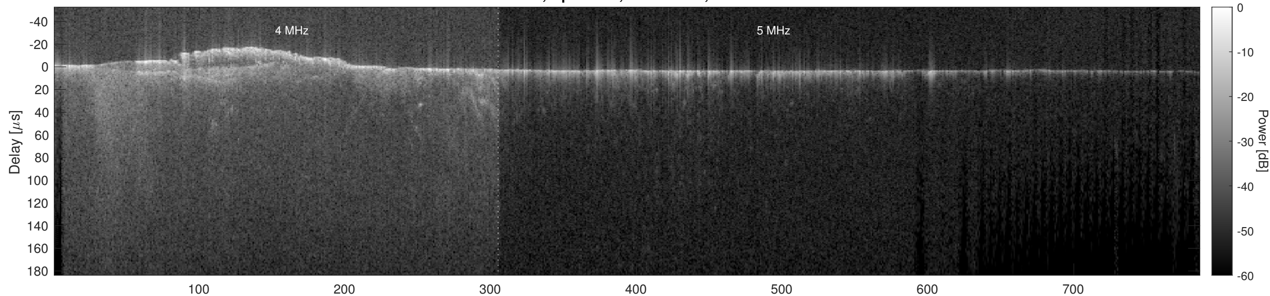
Orbit 9555, Optimized, No Window, Channel 2
