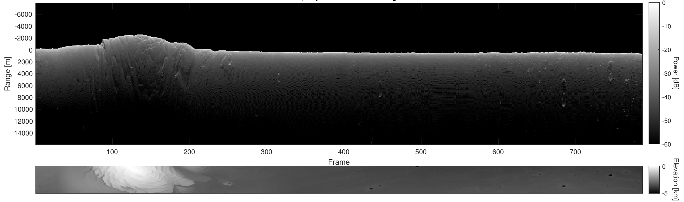
Orbit 9555, Depth-Corrected Cluttergram
