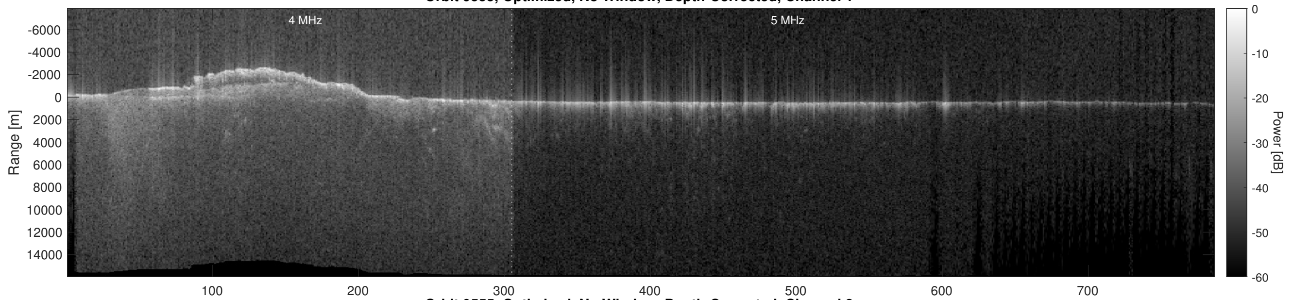
Orbit 9555, Optimized, No Window, Depth-Corrected, Channel 2
