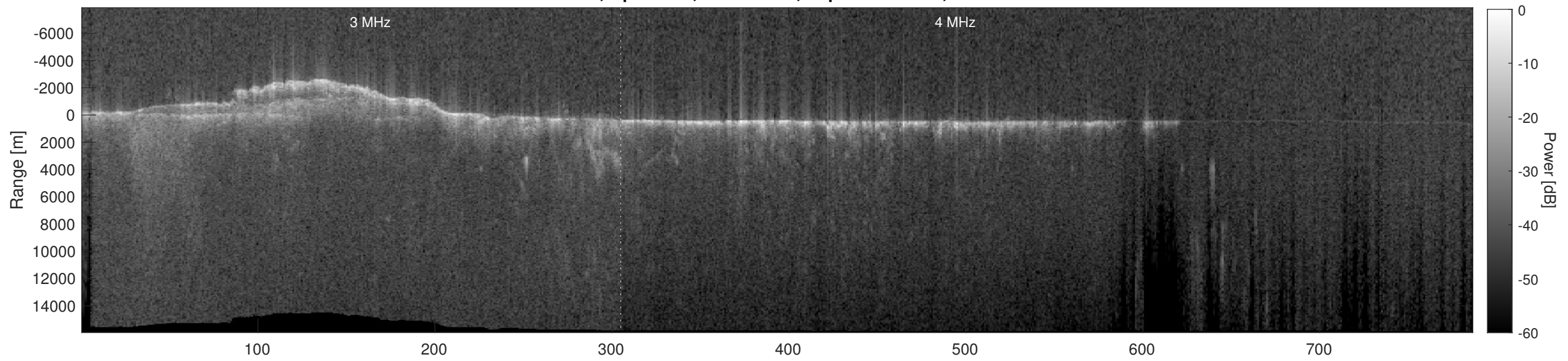
Orbit 9555, Depth-Corrected Cluttergram
