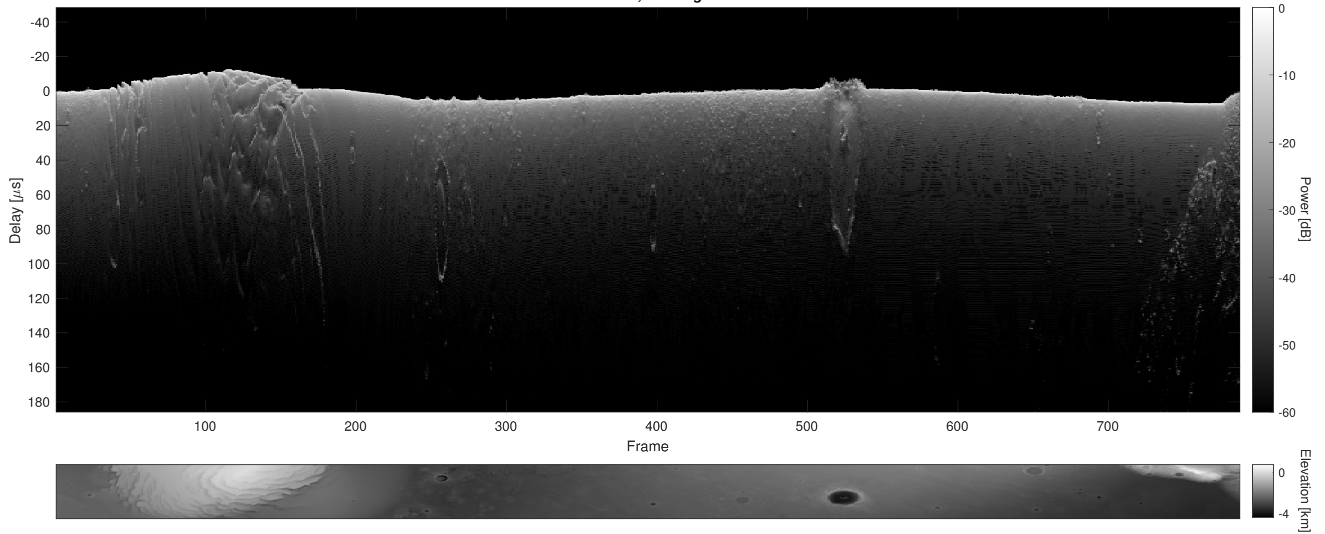
Orbit 9556, Cluttergram
