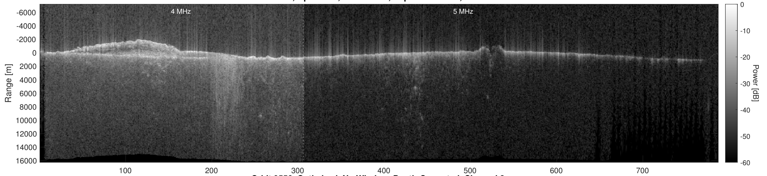
Orbit 9556, Optimized, No Window, Depth-Corrected, Channel 2
