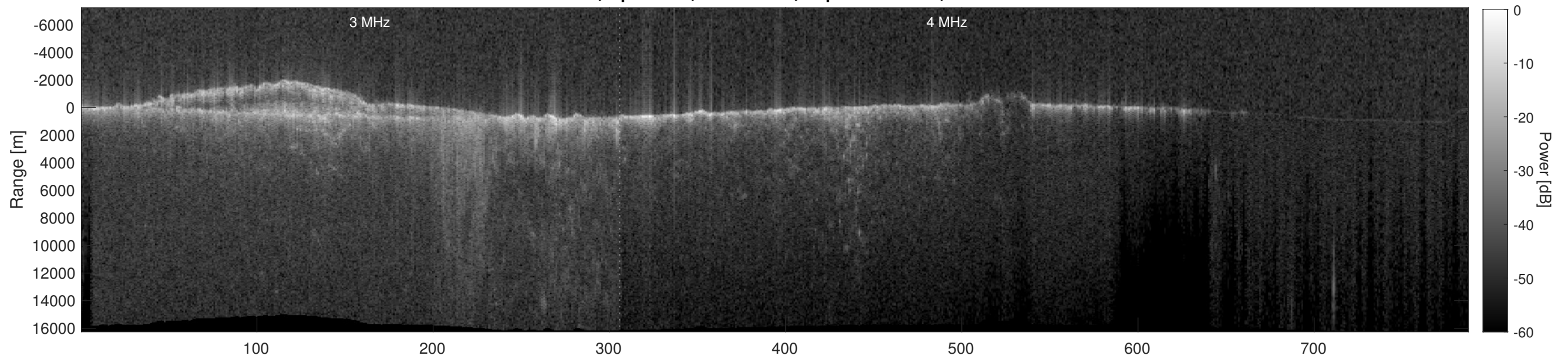
Orbit 9556, Depth-Corrected Cluttergram
