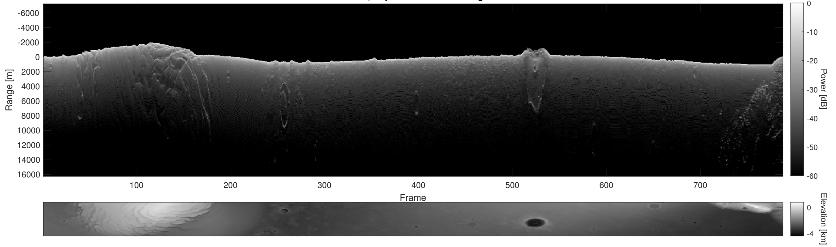
Orbit 9556, Depth-Corrected Cluttergram
