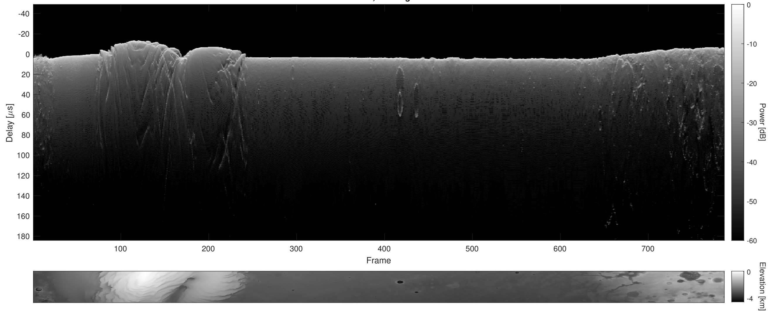
Orbit 9558, Cluttergram
