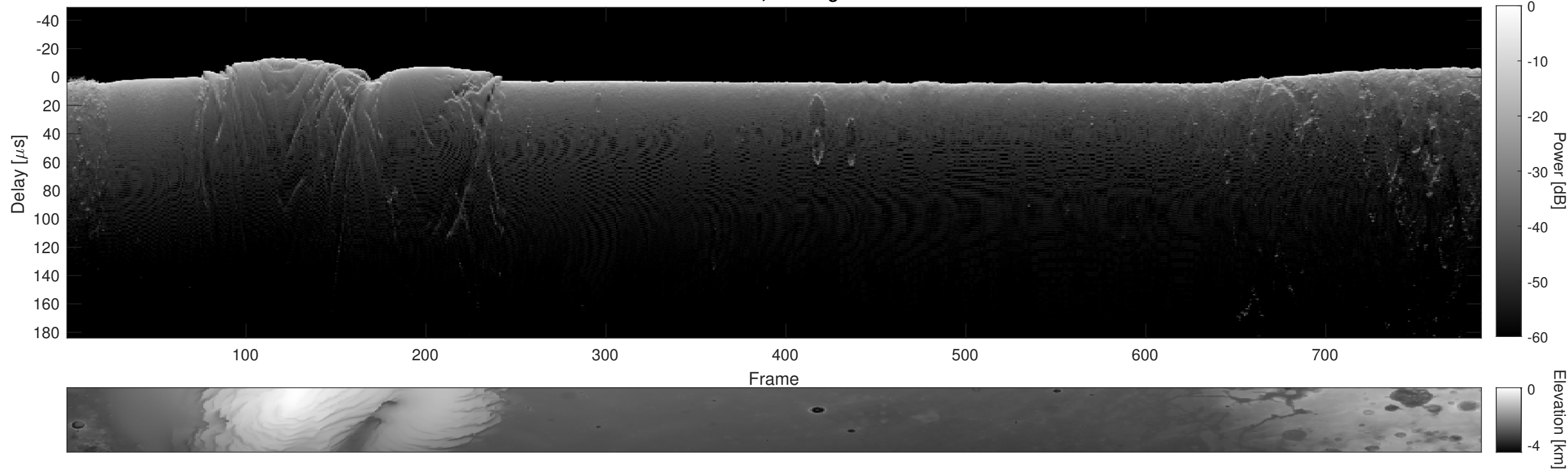
Orbit 9558, Cluttergram
