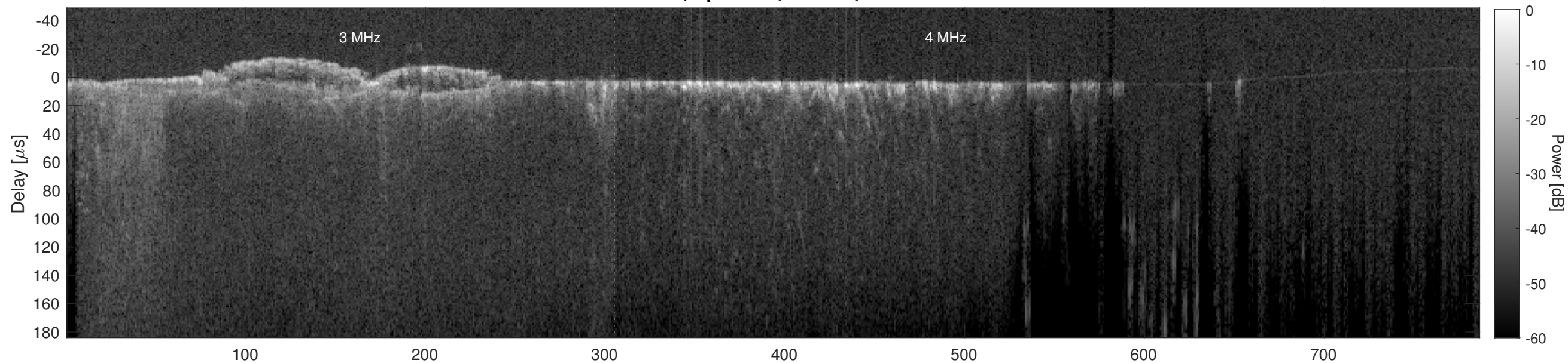
Orbit 9558, Cluttergram
