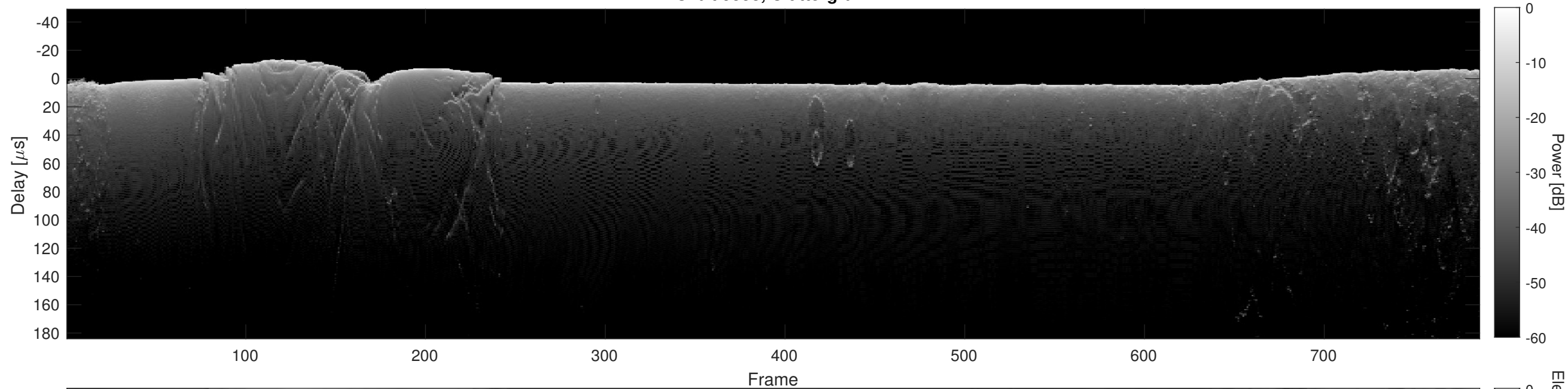
Orbit 9558, Cluttergram
