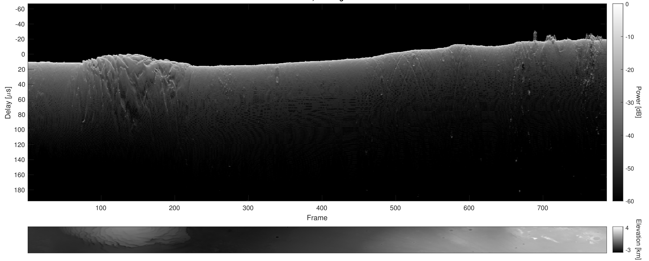
Orbit 9559, Cluttergram
