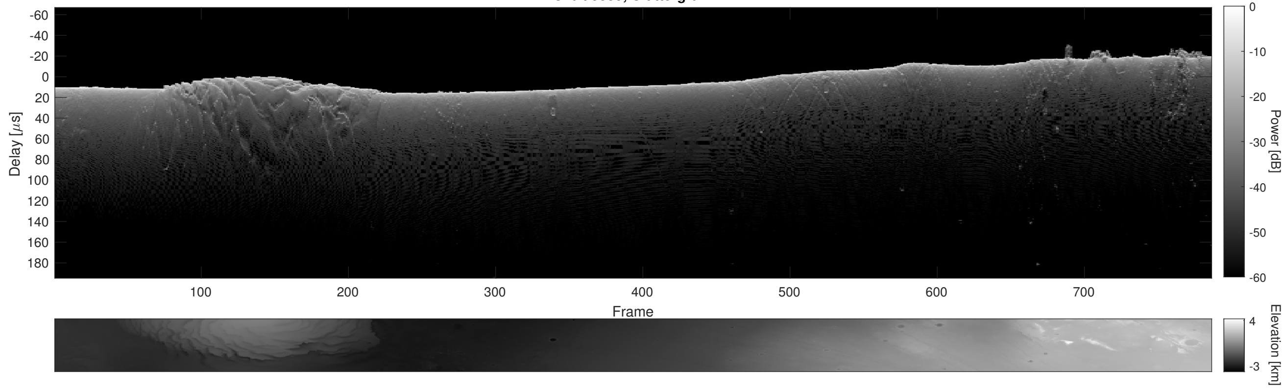
Orbit 9559, Cluttergram
