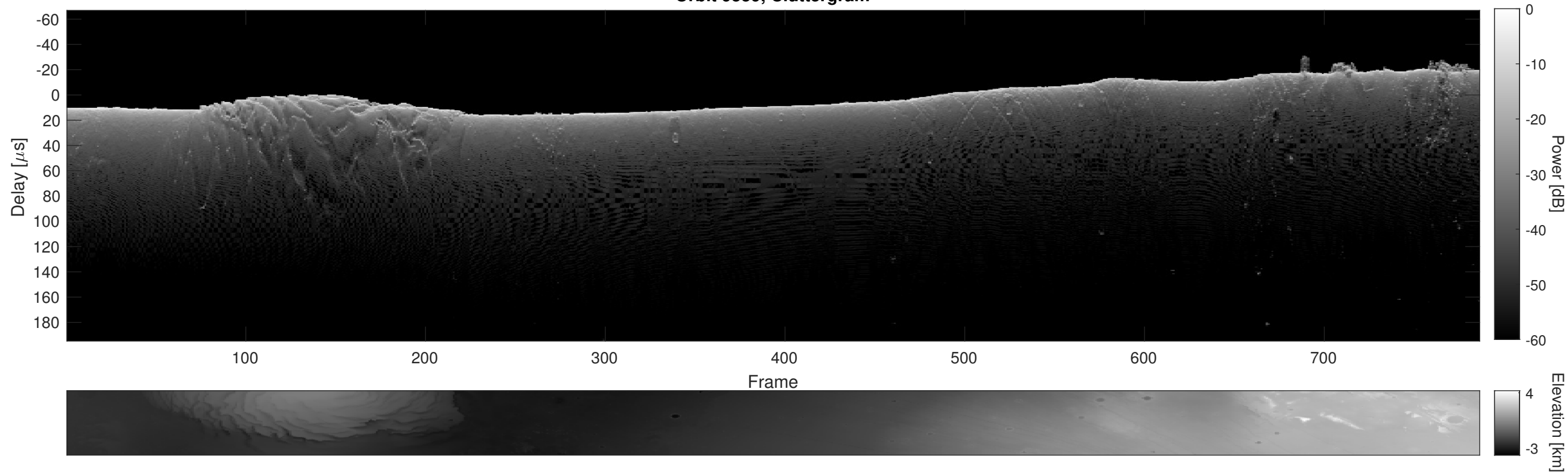
Orbit 9559, Cluttergram
