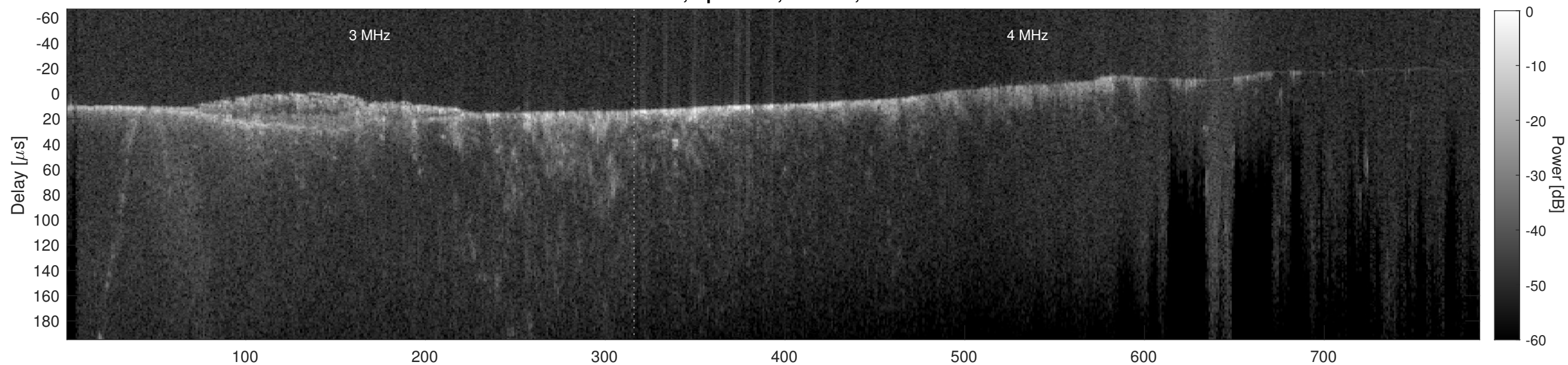
Orbit 9559, Cluttergram
