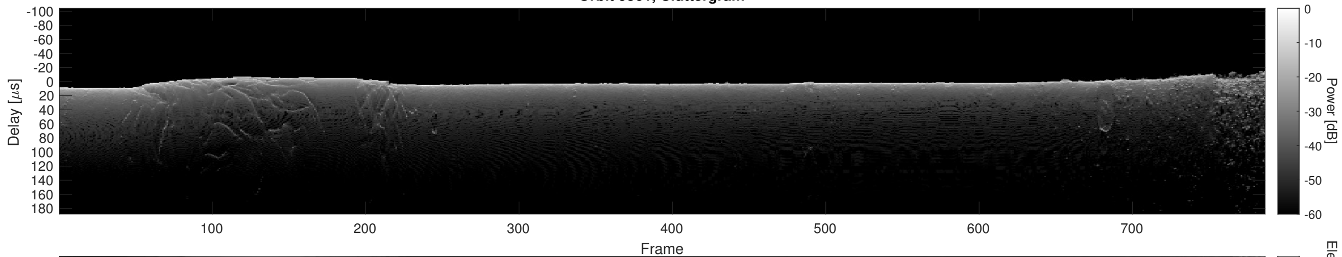
Orbit 9561, Cluttergram
