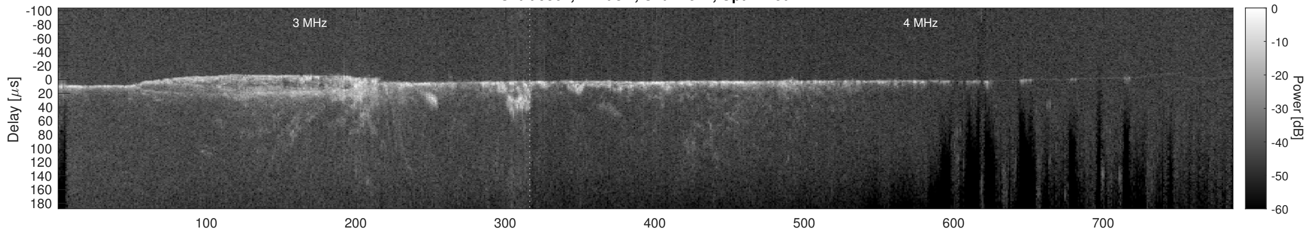
Orbit 9561, Cluttergram
