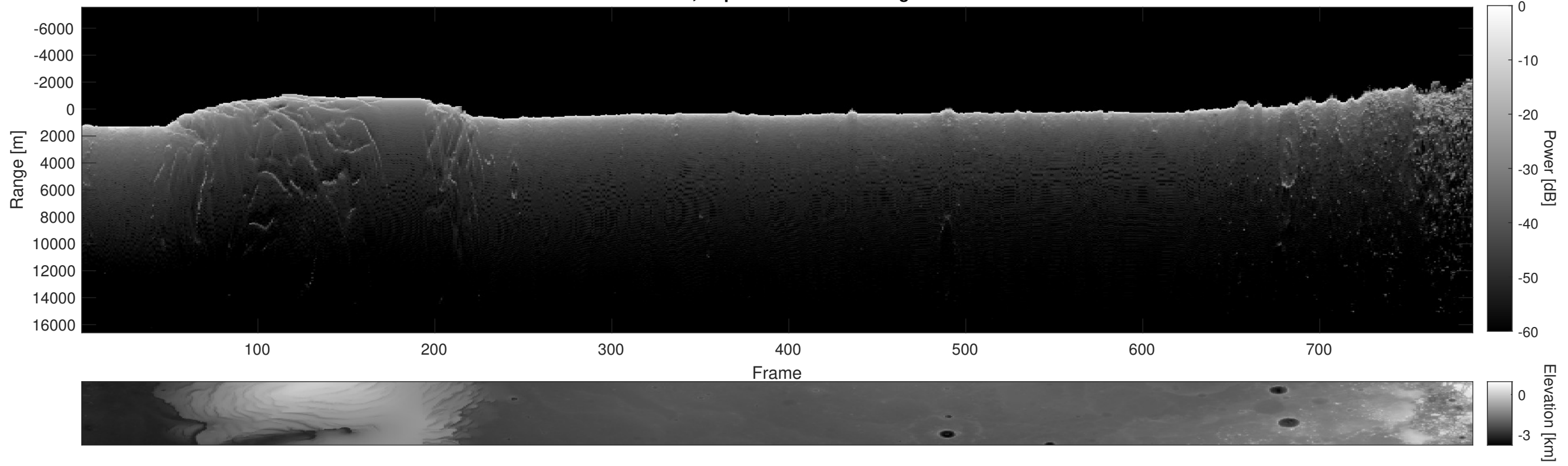
Orbit 9561, Depth-Corrected Cluttergram
