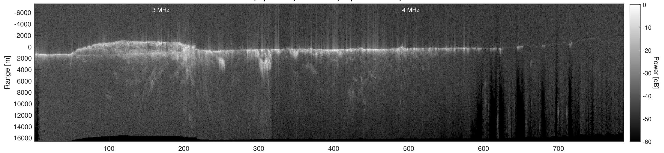
Orbit 9561, Depth-Corrected Cluttergram
