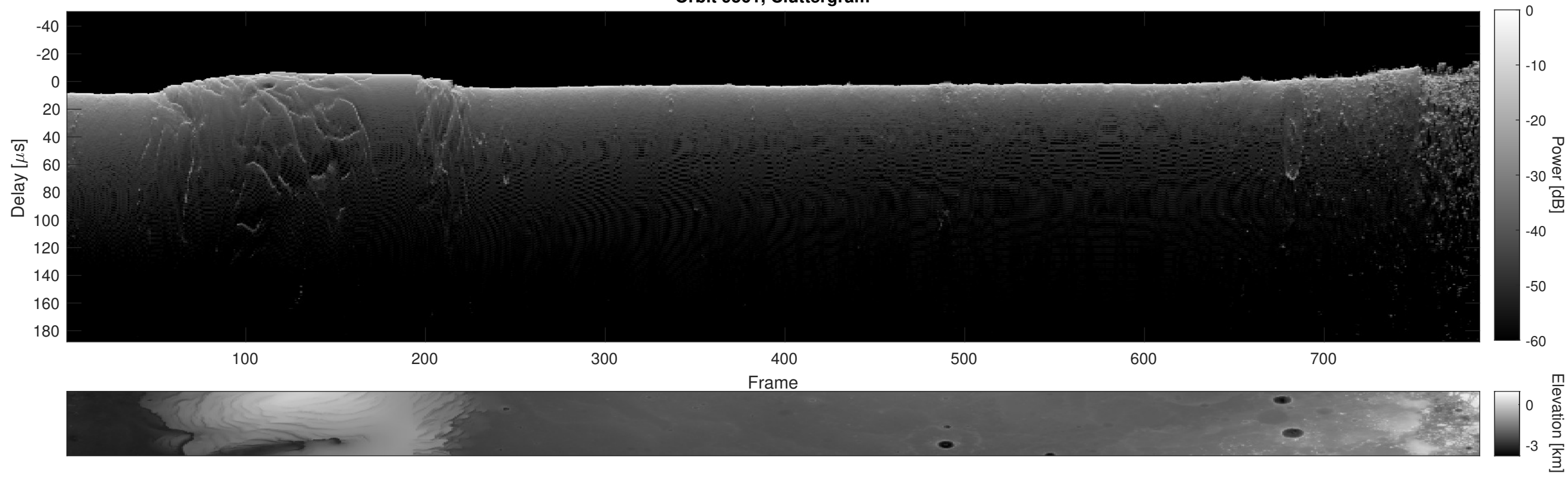
Orbit 9561, Cluttergram
