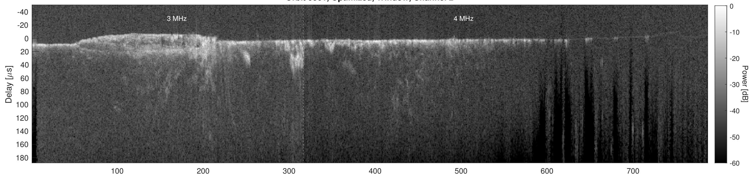
Orbit 9561, Cluttergram
