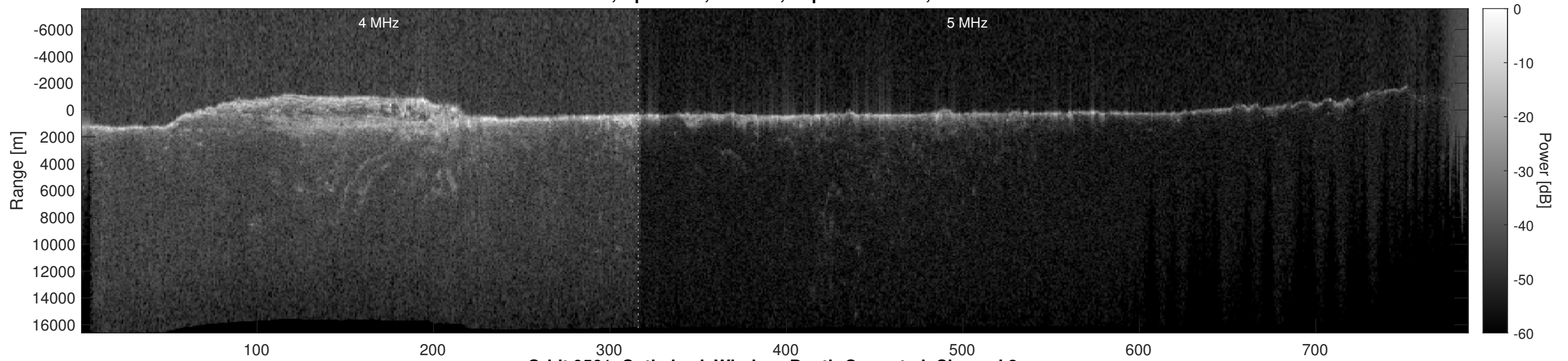
Orbit 9561, Optimized, Window, Depth-Corrected, Channel 2
