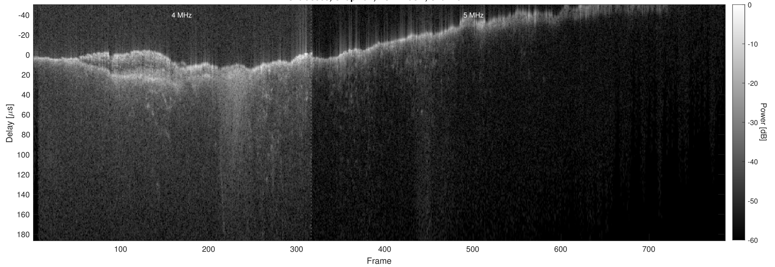
Orbit 9563, Chapman, No Window, Channel 2
