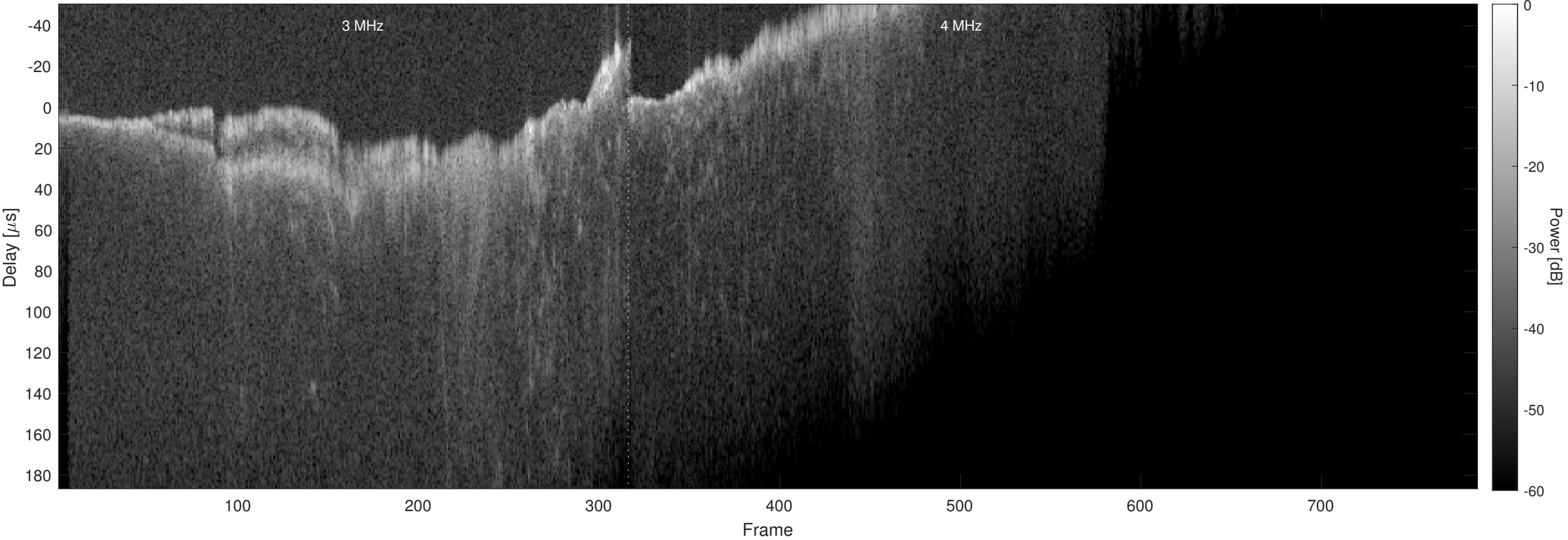
Orbit 9563, Chapman, Window, Channel 2
