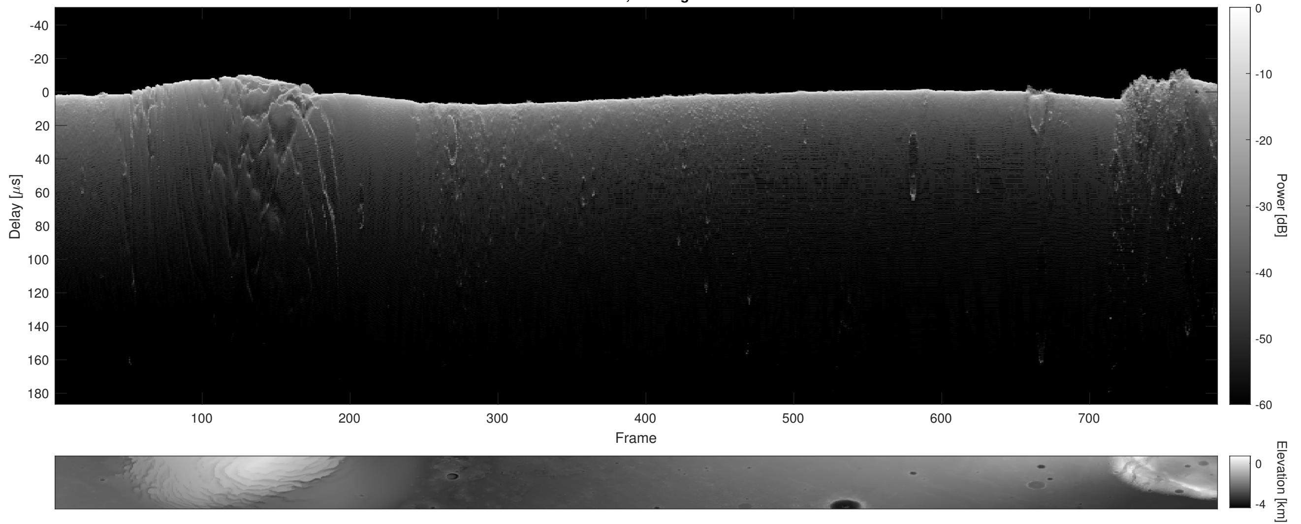
Orbit 9563, Cluttergram
